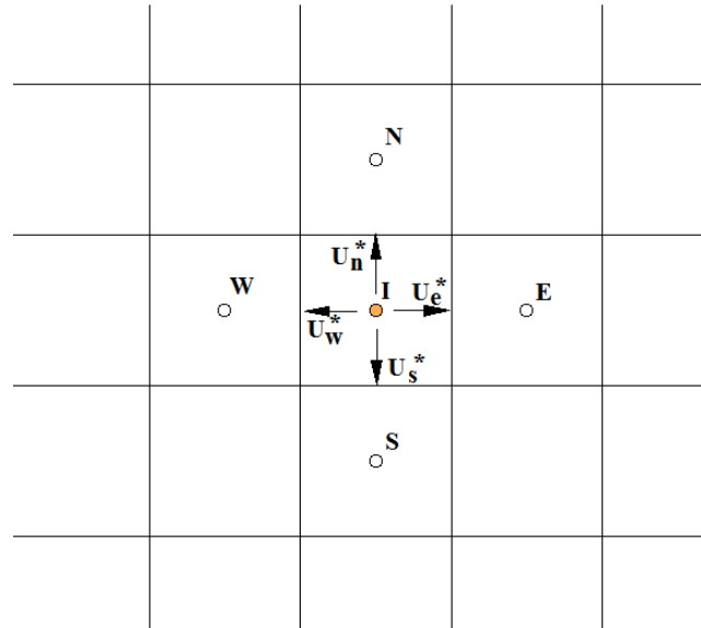
Figure 4-2 A finite-volume Cartesian cell and the cell face fluxes.
