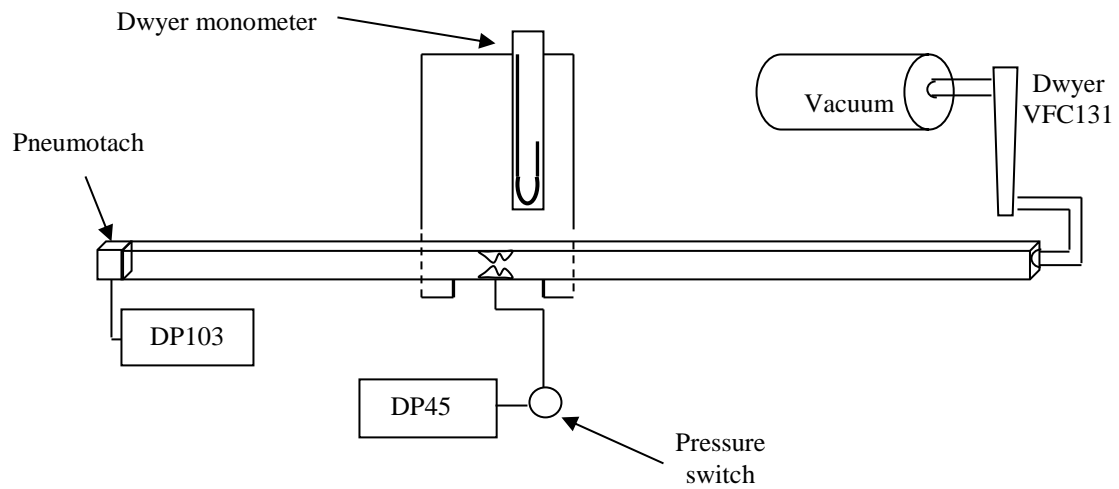
Figure 2-4 A schematic view of the wind tunnel and experimental set up
