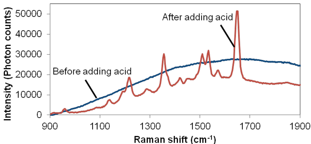
Figure 6.7 Addition of nitric acid promotes interaction between the TAMRA-labeled reporter and the metal nanostructures, enabling the SERS spectrum of TAMRA to be observed
