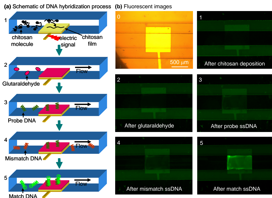
Figure 3-3: DNA hybridization in bioMEMS. (a) Schematic procedure. (b) Fluorescent micrographs.
