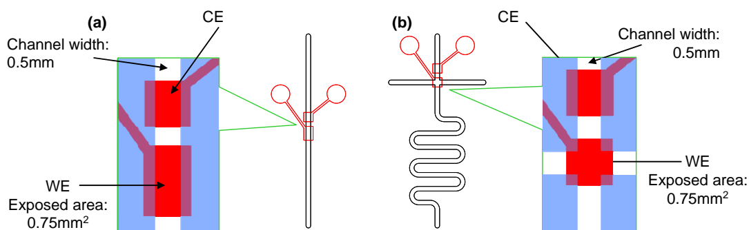
Figure S-1: Working electrodes (WE) were fabricated to match the exposed surface area in both (a) single-channel and (b) cross-channel.
