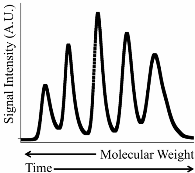
Figure 1.8. Representative GPC chromatogram of narrow molecular weight distribution poly(styrene) standards. Higher molecular weight polymers elute first and are followed by low molecular weight adducts.
