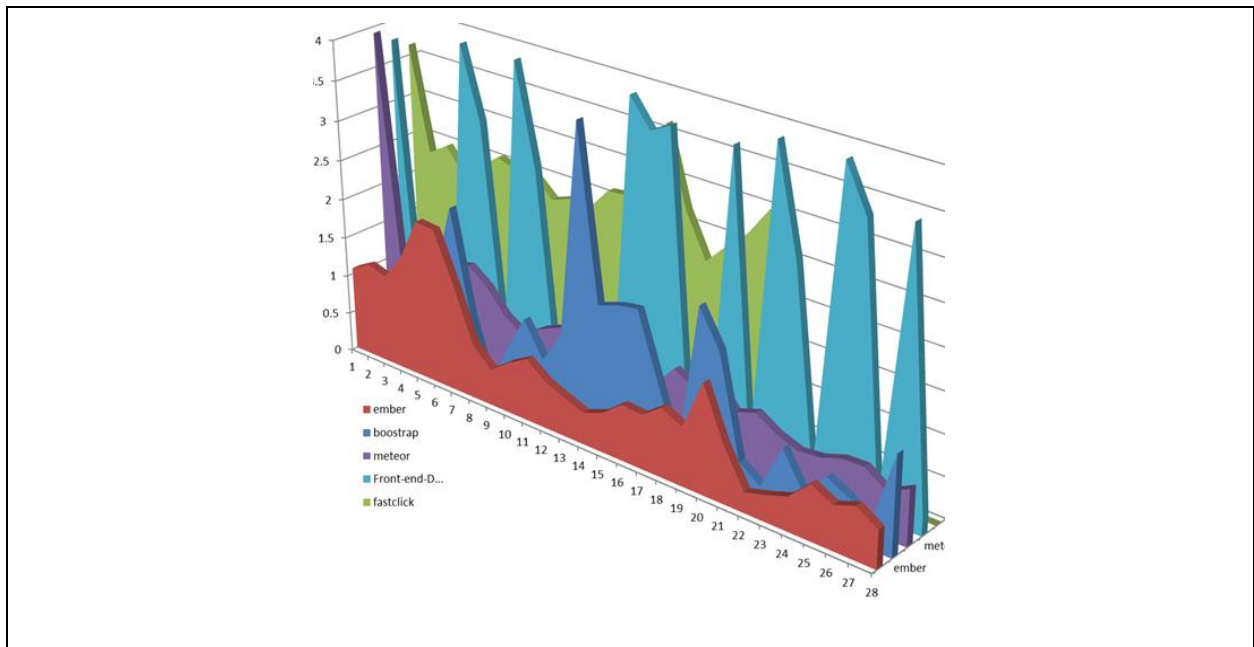
Figure 12. HMM Differences of Cluster Samples
