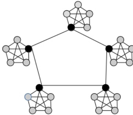
Figure 3.5: Tribal-PSO
