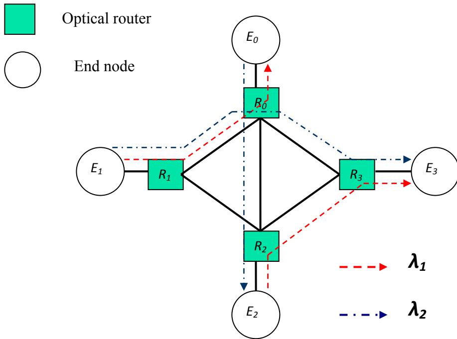
Figure 1.1: Some lightpaths on a physical topology.
