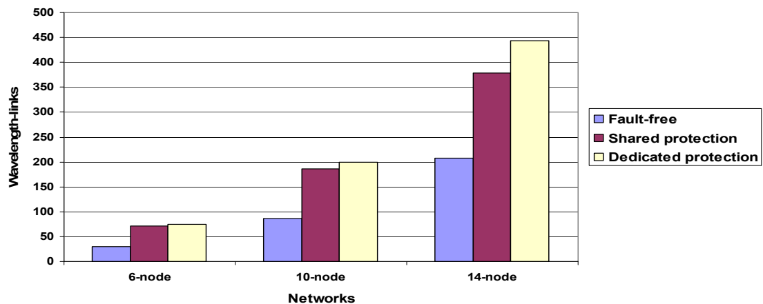
Figure 3.7: Resource requirements vs. network size with |K| = 16 in survivable wavelength continuous networks under LDO model.
