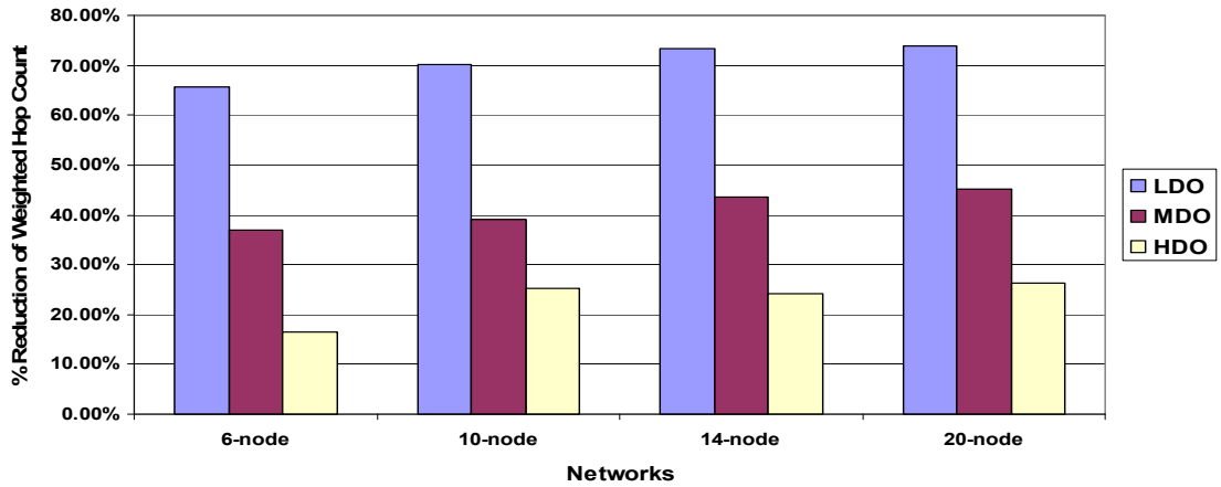
Figure 3.4: Percentage improvement in resource requirements compared to FDO case in fault-free networks with wavelength conversion.
