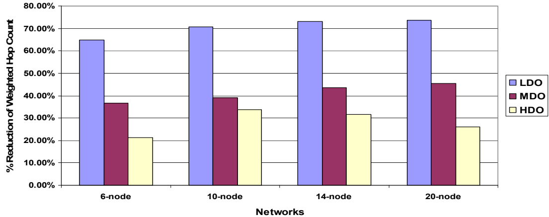
Figure 3.2: Percentage improvement in resource requirements compared to FDO case using ILP1.
