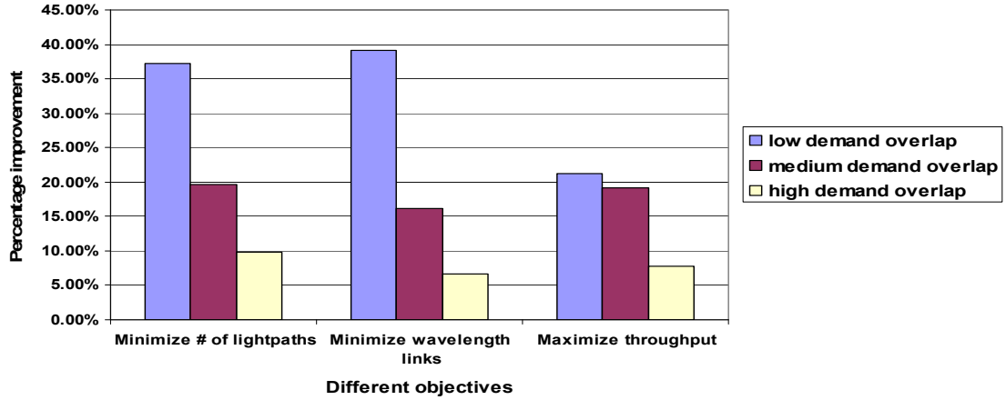
Figure 3.6: Relative improvement with different objective functions.
