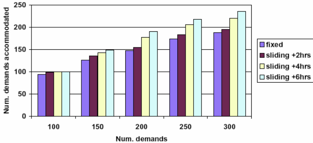
Figure 5.2: Number of demands accommodated using H-SSD for 14-node network.
