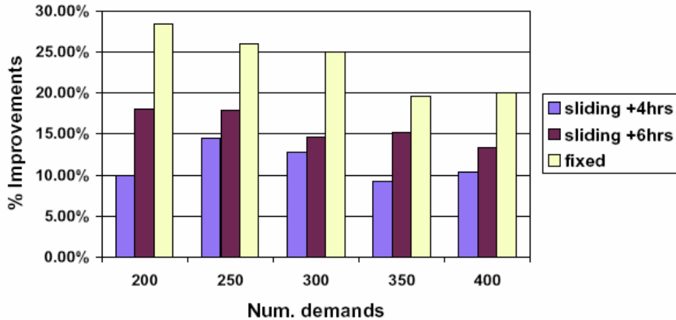
Figure 5.4: Percentage improvements in the number of demands accommodated by the network, obtained using H-SSD compared to continuous scheduled traffic model.
