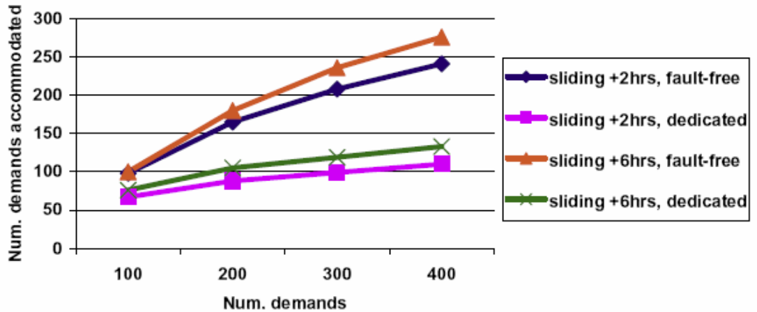
Figure 5.7: Comparison of the number of accommodated demands for fault-free networks versus dedicated protection.
