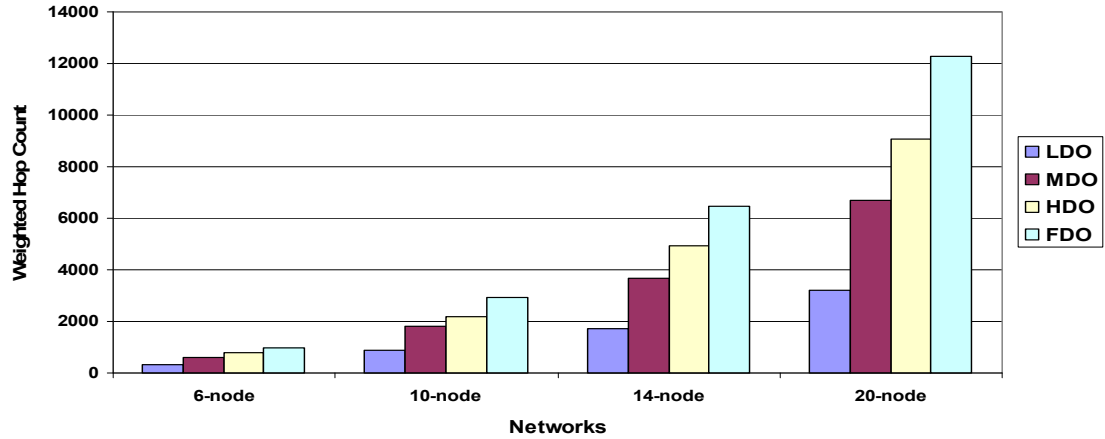
Figure 3.1: Resource requirements vs. network size in fault-free networks without wavelength conversion.
