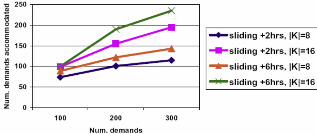
Figure 5.5: Effect of increasing fiber capacity or window size on a 14-node network.
