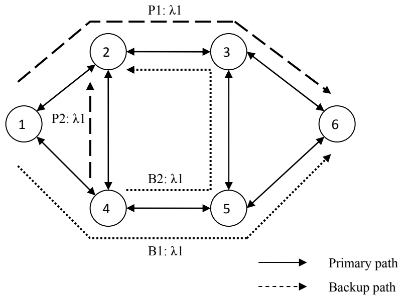
Figure 2.2: Shared path protection.
