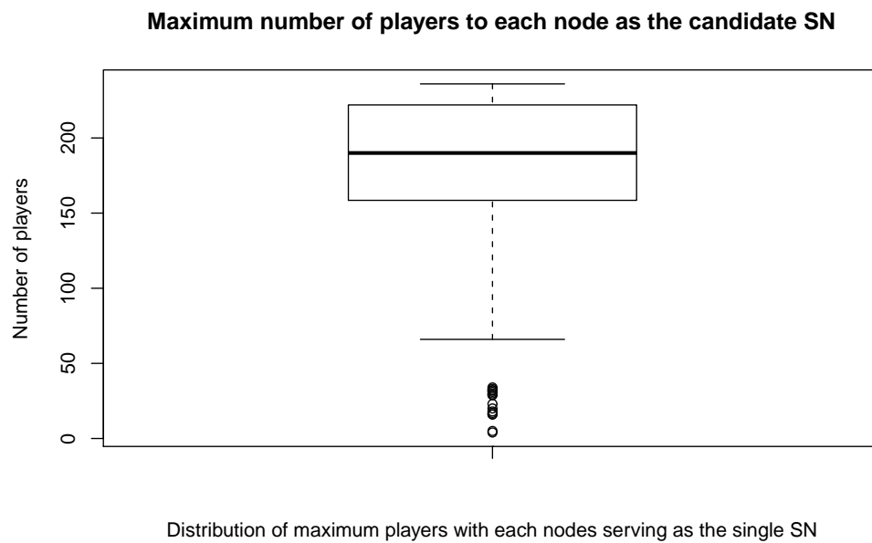
Figure 5.19: Maximum number of players each node supports if serving as the SN. This is based on a 180 ms RTT required to connect to the SN.
