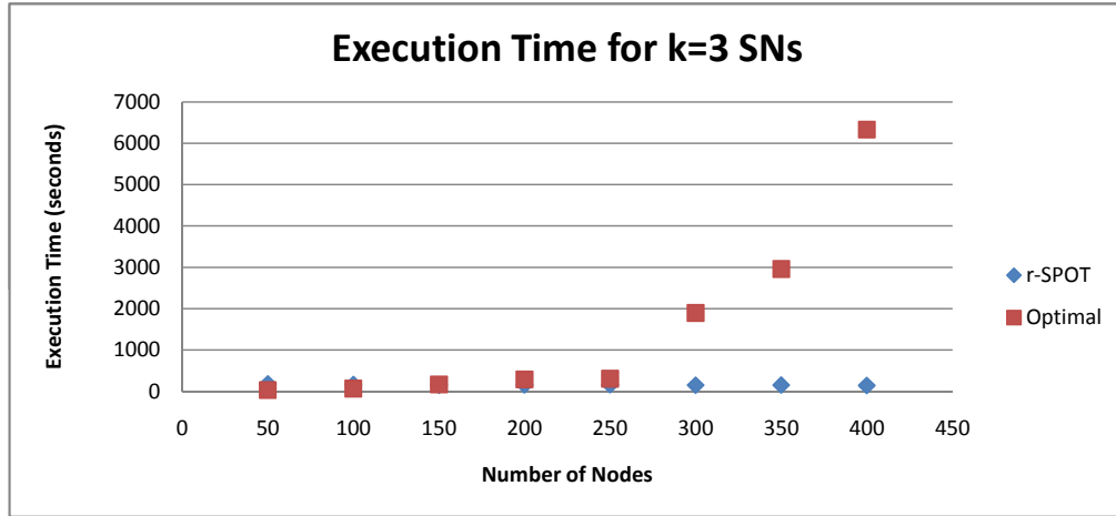
Figure 4.11: Total time to place three SNs in r -SPOT algorithm compared to the optimal placement.
