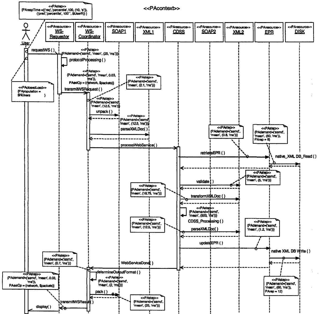
Figure 4.2 Annotated UML Sequence Diagram for Web Services Invocation
