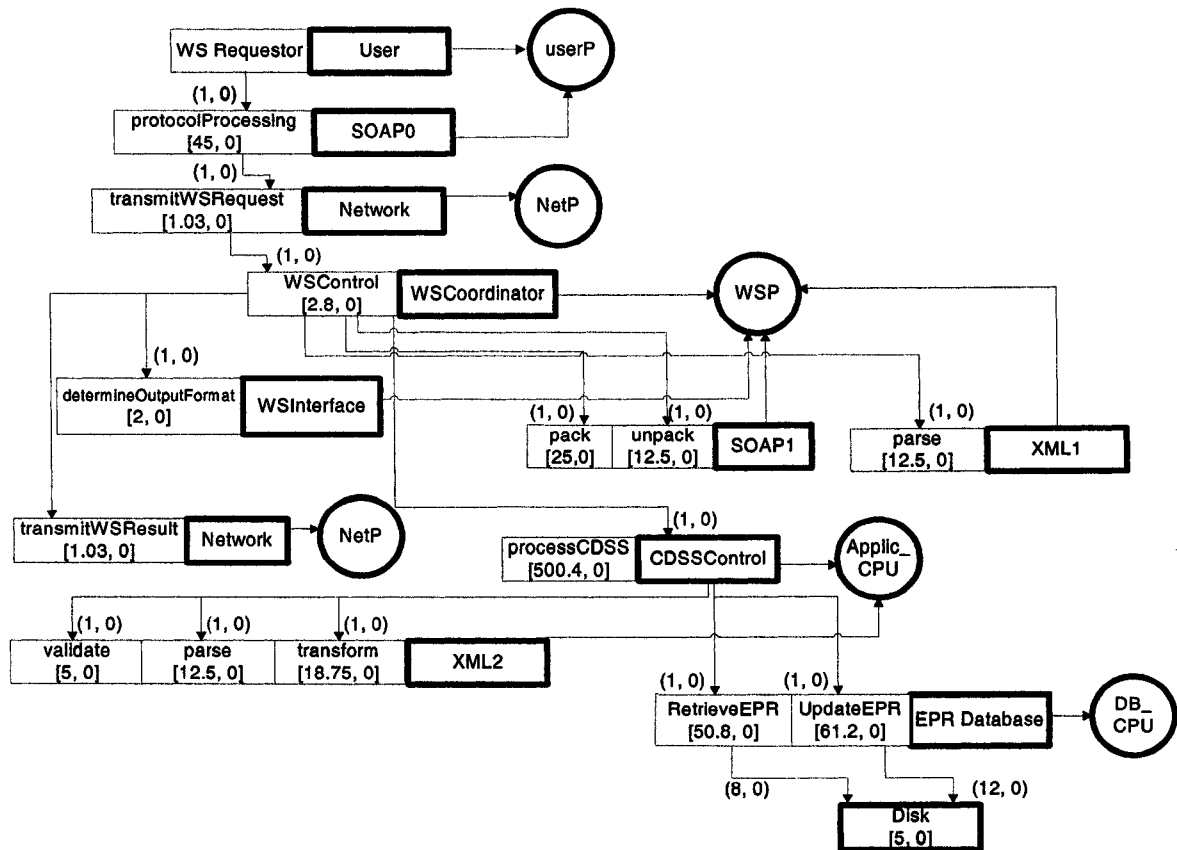
Figure 4.3 Layered Queuing Network Model for Web Services Invocation
