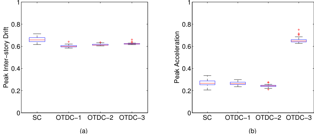
Figure 6.3: Structural Response under Wireless Building Control: (a) Peak Inter-story Drift; (b) Peak Acceleration.
