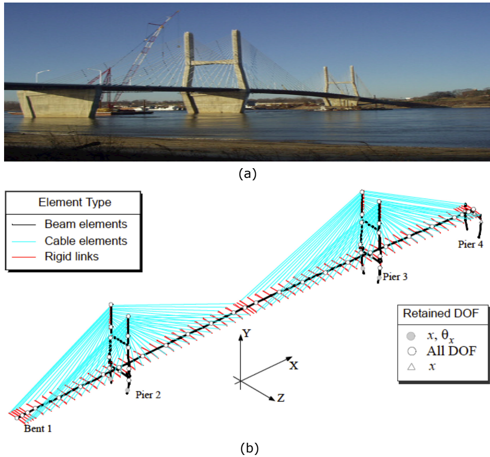
Figure 4.7: Cape Girardeau model in WCPS: (a) the Cape Girardeau bridge; (b) Simulink model of the Cape Girardeau bridge [10].
