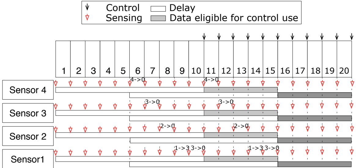
Figure 5.2: Example of OTDC-1 with UDS scheduler.
