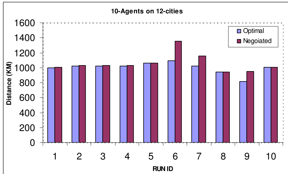
Figure 4.7: Total travel distance to meeting by 10 agents
