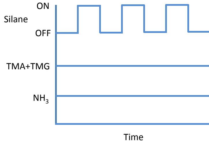
Figure 4. 1 Precursor flow time for silicon doping modulation AlGaIn.
