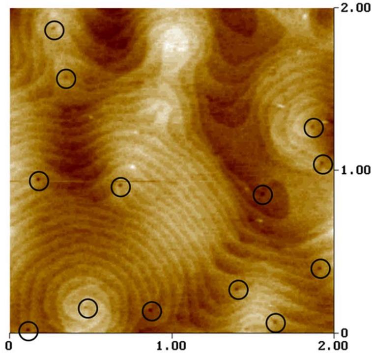
Figure 3. 7 AFM image of superlattice template (EPD \sim 3 \times 10^8 cm ^{-2} ).
