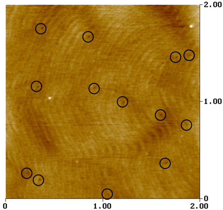
Figure 4. 6 AFM image of sample B (EPD \sim 3.5 \times 10^8 cm ^{-2} ).
