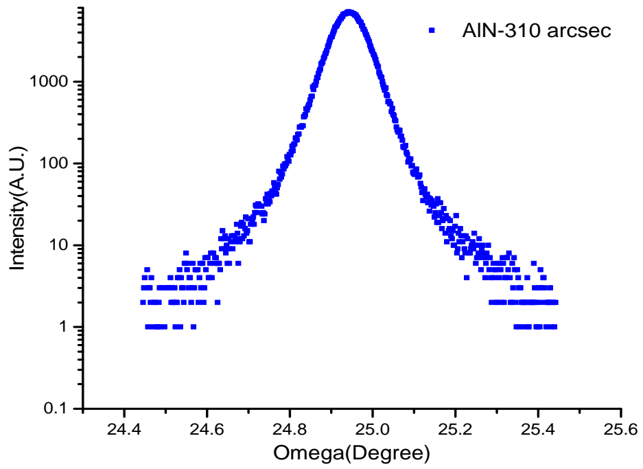
Figure 3. 1 XRD(102) scan of AlN template.
