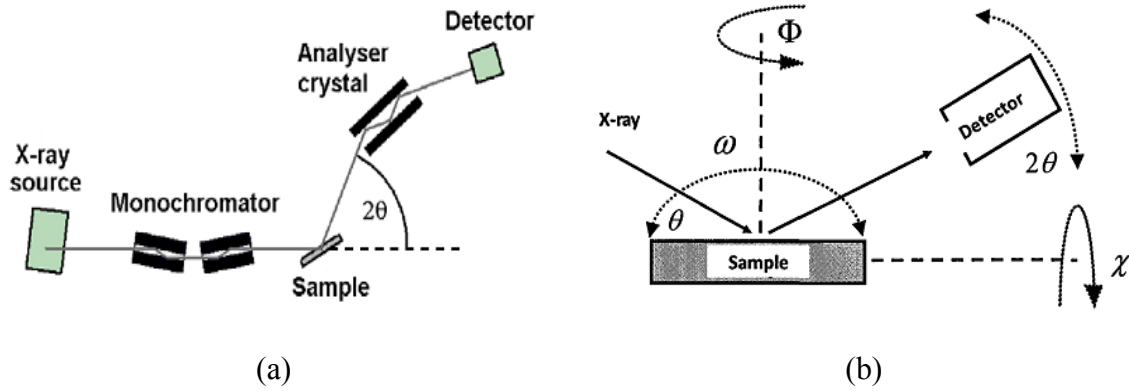
Figure 2. 8 Scheme of high resolution X-ray diffractometer. [106]
