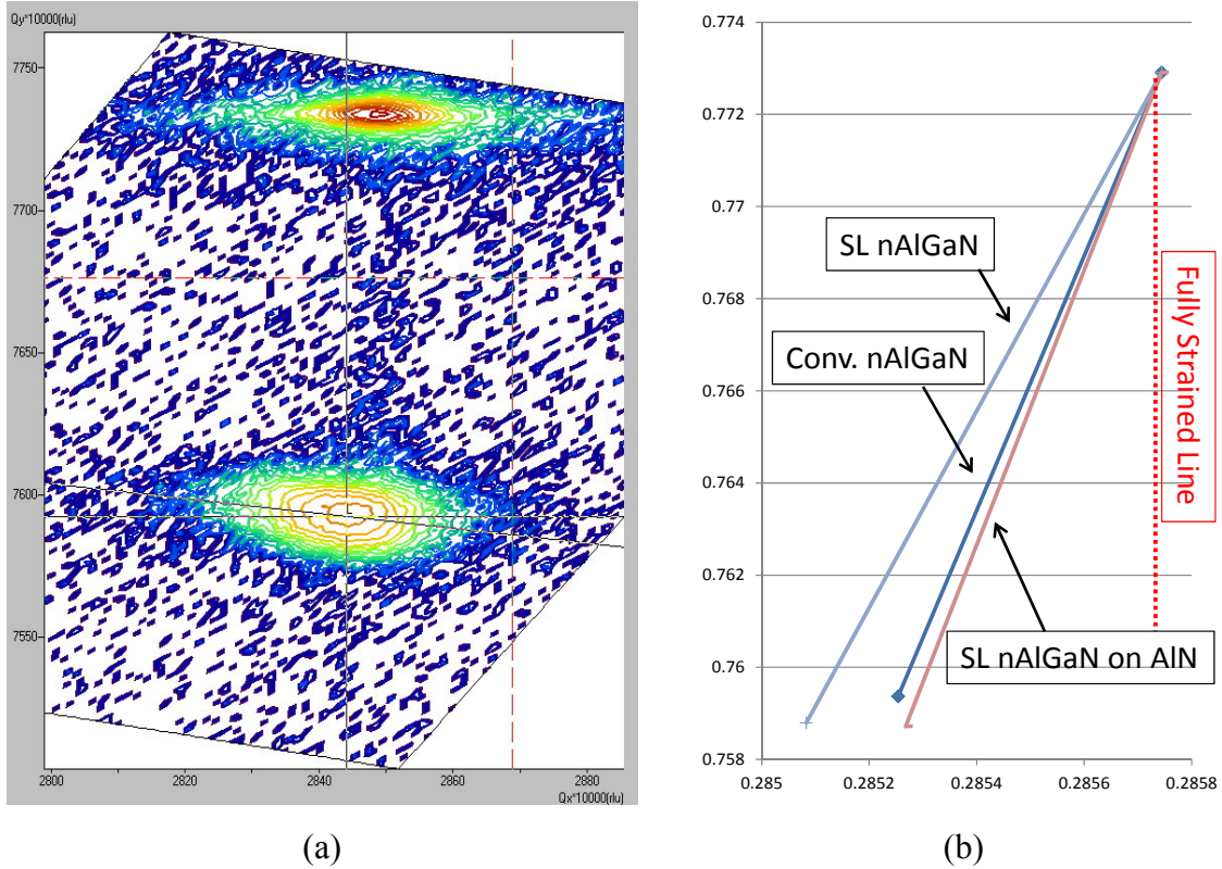
Figure 3. 21 XRD Reciprocal space mapping.
