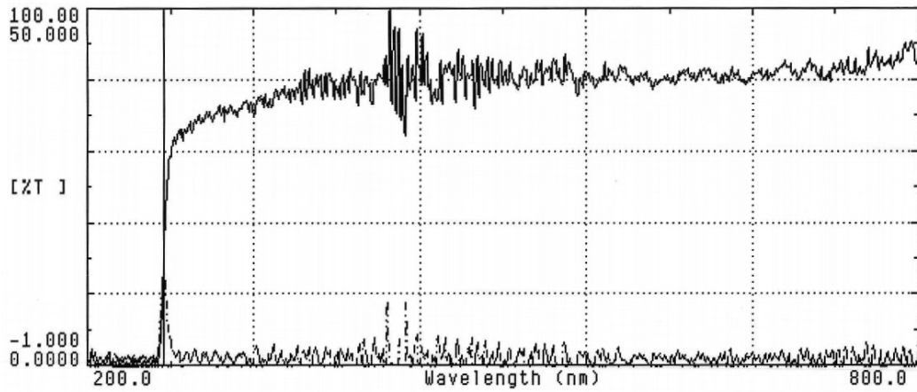
Figure 3. 16 Transmission measurement of superlattice nAlGaN on AlN template.
