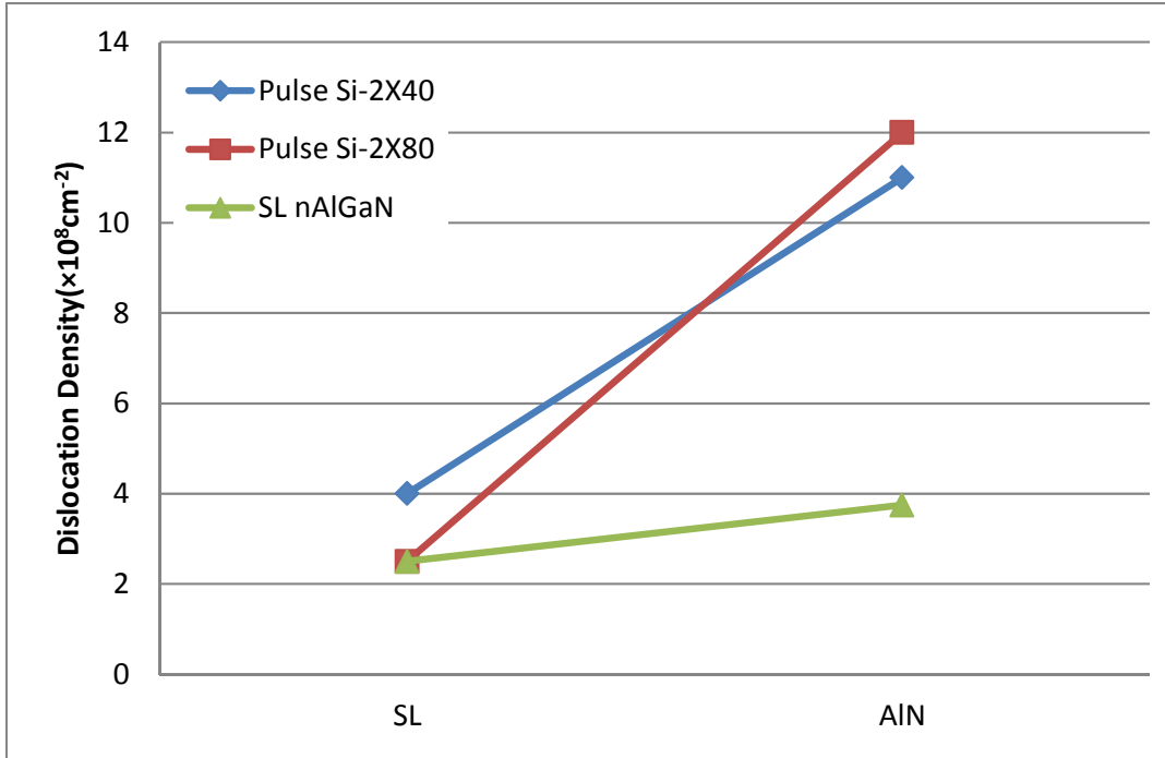
Figure 4. 22 Dislocation densities of nAlGaIn samples on different template.
