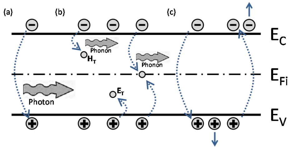
Figure 1. 2 Band Diagram illustrating recombination: (a) radiative (b) non-radiative via deep levels and (c) non-radiative via Auger processes.
