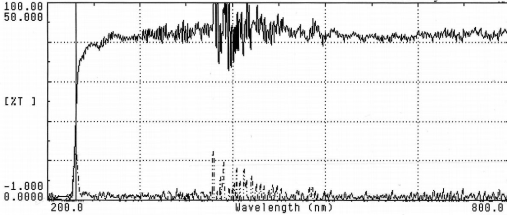
Figure 3. 8 Absorption edge calibration of AlN/AlGaIn superlattice.
