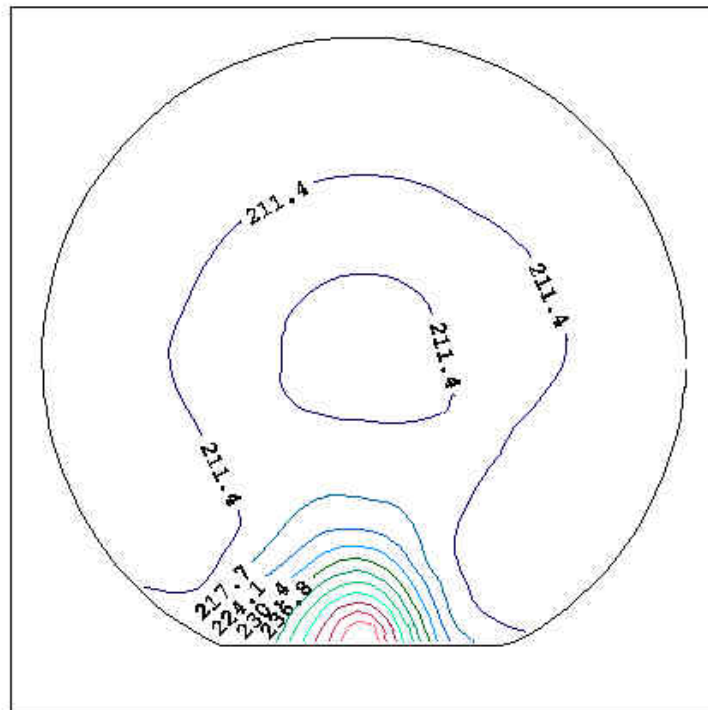
Figure 3. 17 Sheet resistance mapping of superlattice nAlGaN on AlN template.
