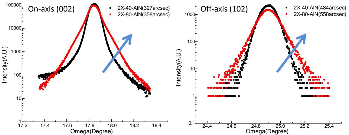
Figure 4. 20 XRD (002) and (102) scans of silicon doping modulation AlGaN samples on AlN template.
