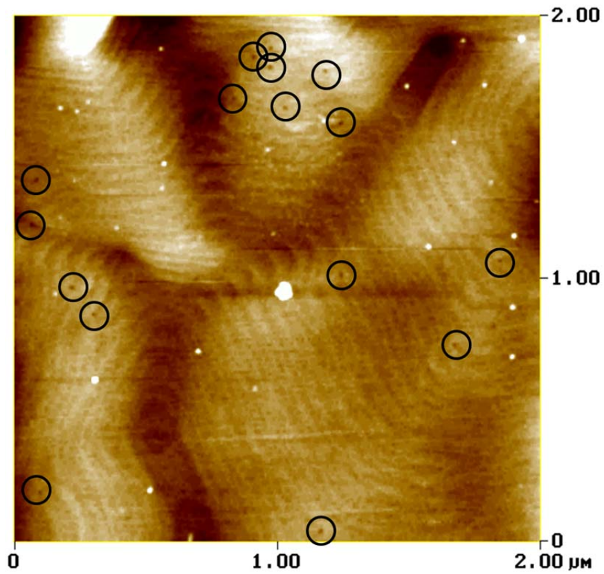
Figure 4. 5 AFM image of sample A (EPD \sim 4 \times 10^8 cm ^{-2} ).
