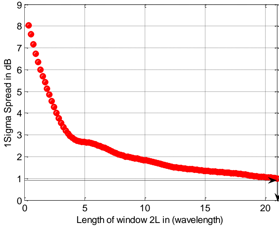
Figure 4.16 Spread of estimated local means as a function of 2L when d_{LA} was 18.28 m. One-dB threshold indicated by arrows.
