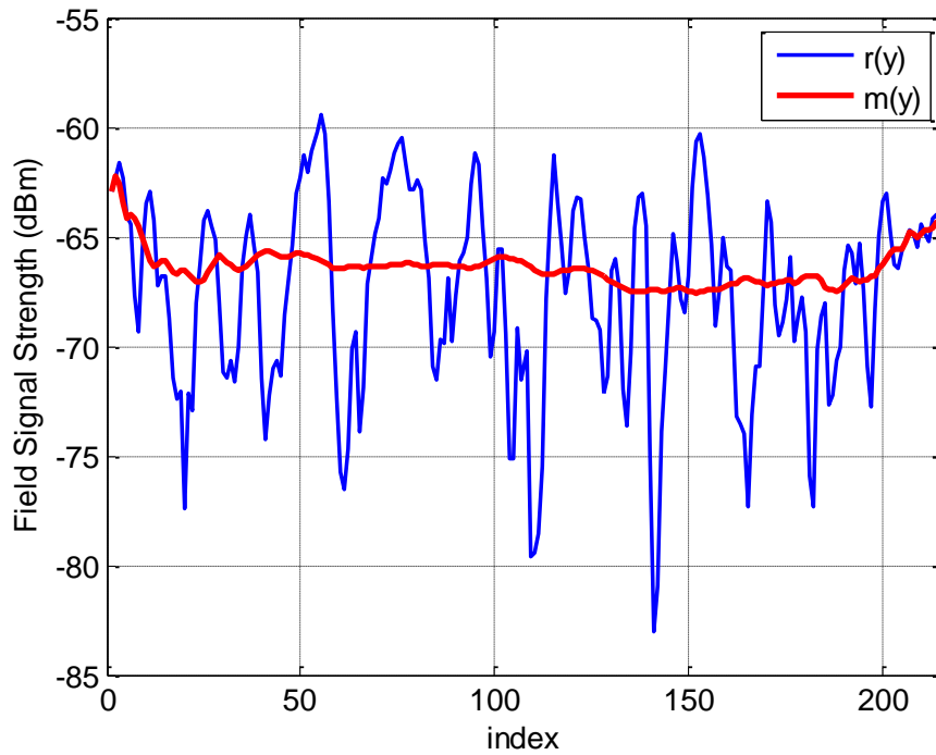
Figure 4.17 Signal envelope using optimum averaging window length at d_{LA} = 18.28 m.
