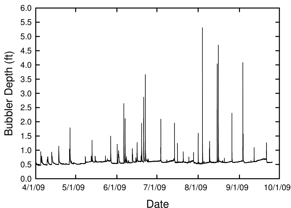
Figure 4.3: Colonial Hills Depth Time Series
