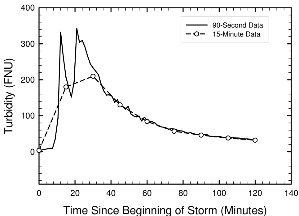
Figure 4.1: Comparison between 15 minute and 90 minute Data (8/4/2009 Event at Colonial Hills)
