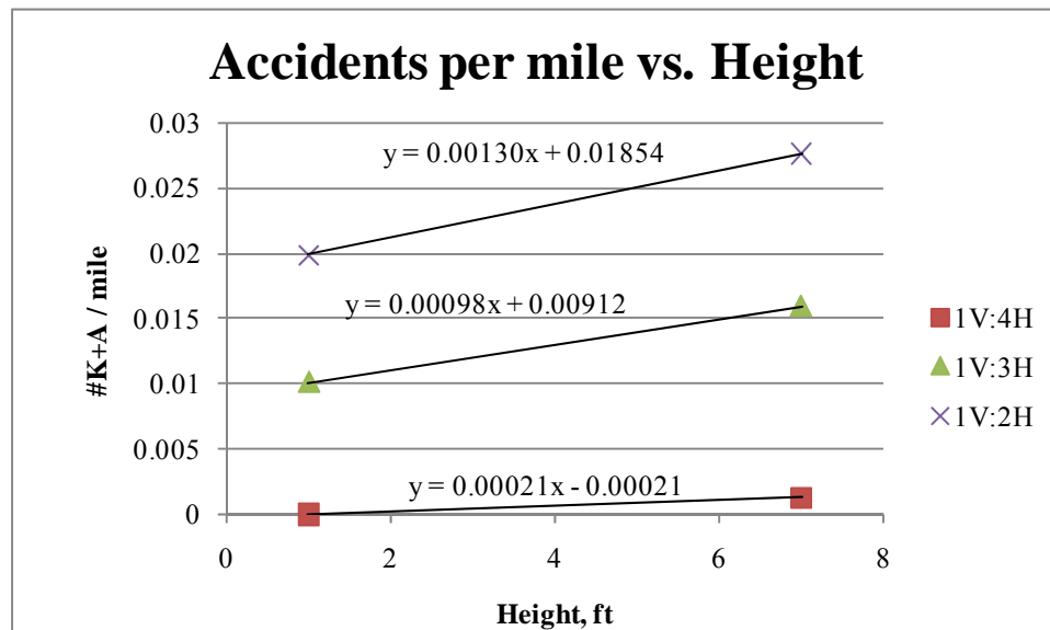
Figure 5. Accident Rates for Foreslopes
