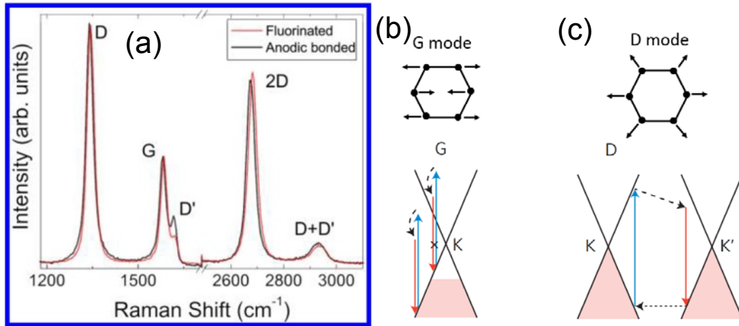
Figure 2.9 (a) Raman spectra of fluorinated and anodic bonded graphene depicting peaks of interest in 1200 to 3000 \text{cm}^{-1} range in a defective graphene [41]. (b) G band resulting from in-plane C-C band stretching of the ring and is characteristic of \text{sp}^2 carbon system. Electron excitation and phonon generation is shown as resonance process in the E-k diagram of graphene. (c) The radial breathing mode responsible for D peak. It involves intervalley phonon and defect scattering [43].
