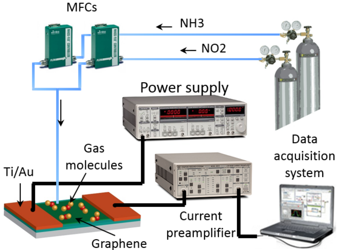
Figure 3.15 Schematic of amperometric measurement set up for chemical sensing where calibrated test gases (20 ppm NO 2 , 550 ppm NH 3 ) are delivered to sensor under test. The current as a function of time is measure by current preamp and recorded by data acquisition system.
