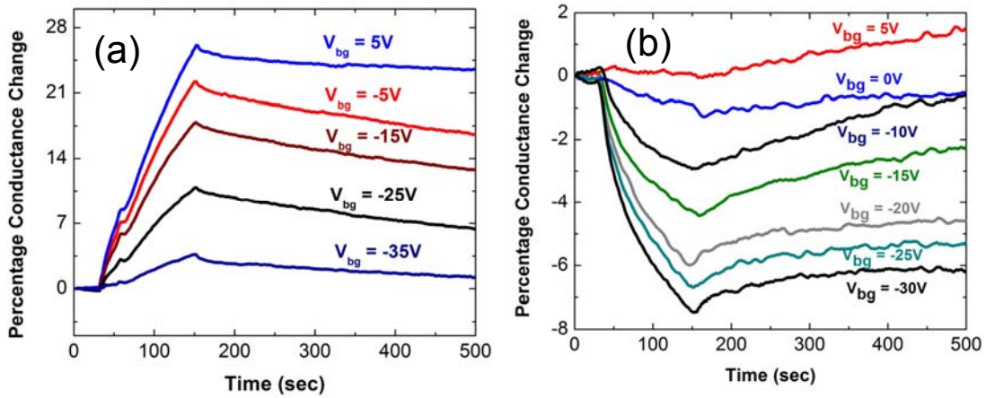
Figure 3.17 Variation of back gated graphene sensor response for (a) 20 ppm \text{NO}_2 exposure with the increase in gate bias from negative to positive values and (b) 550 ppm \text{NH}_3 exposure with the gate bias change from negative to positive values.
