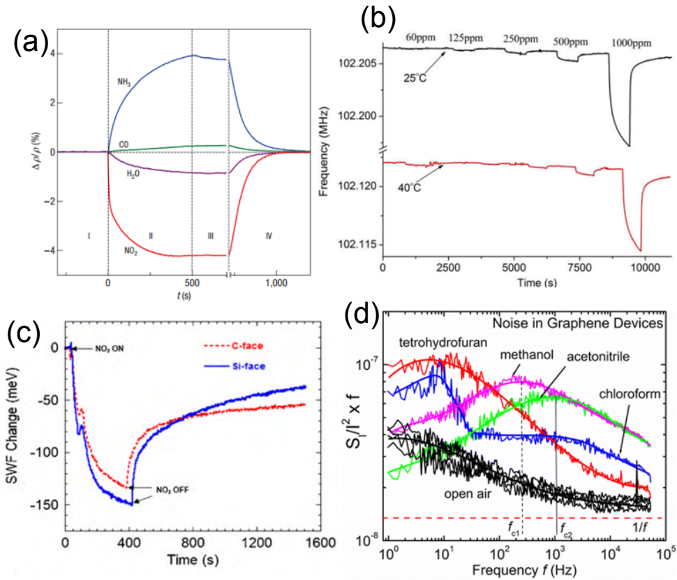
Figure 3.2 Reported sensing modalities of graphene based gas and vapor sensors. Change in (a) conductivity by NO 2 , NH 3 and H 2 O [24], (b) frequency of SAW by CO [99], (c) SWF by NO 2 [85], and (d) unique 1/f noise spectrum of VOCs [88].
