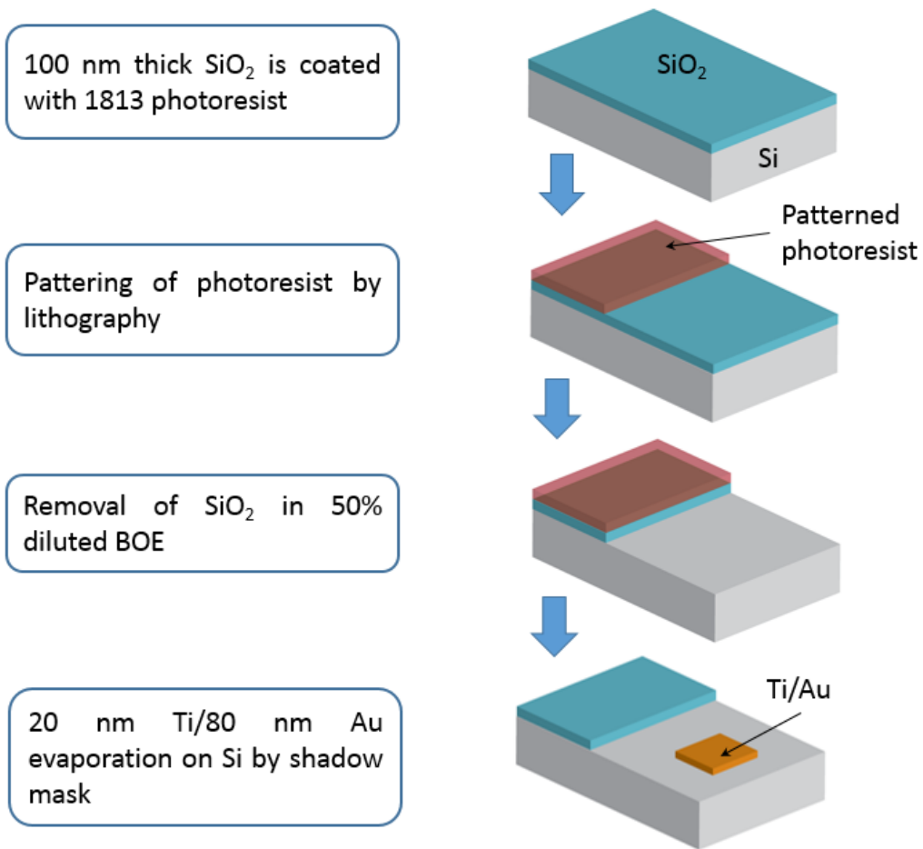
Figure 4.5 The processing steps for the patterning SiO 2 /Si substrate and deposition of metal contacts on Si.
