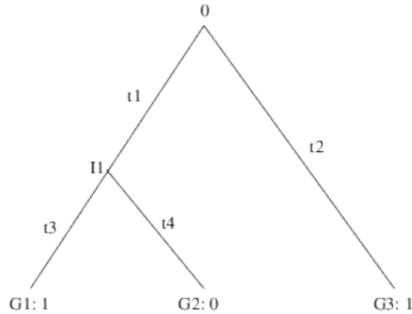
Figure 5.1 A phylogenetic topology of three genomes. The 0 or 1 following the leaf label represent absence or presence of a gene adjacency.
