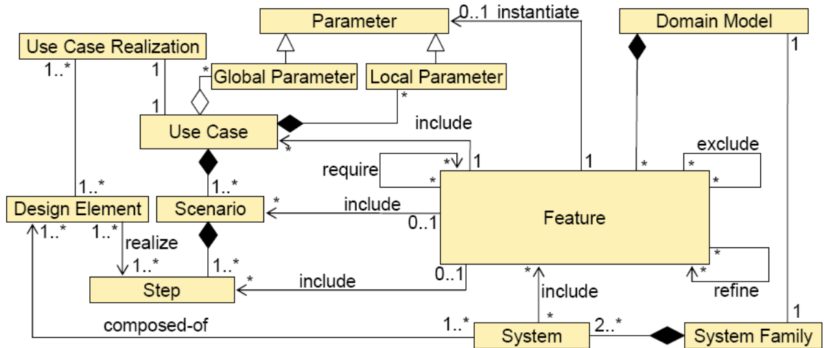
Figure 4.3: PLUSS meta-model [24]
