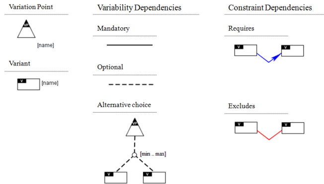
Figure 2.4: OVM notation
