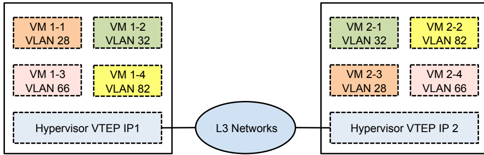
Figure 2.9: Virtual Machines on different VLANs
