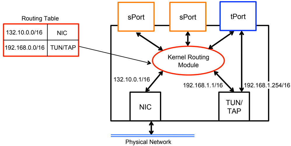
Figure 6.17: Host Interfaces
