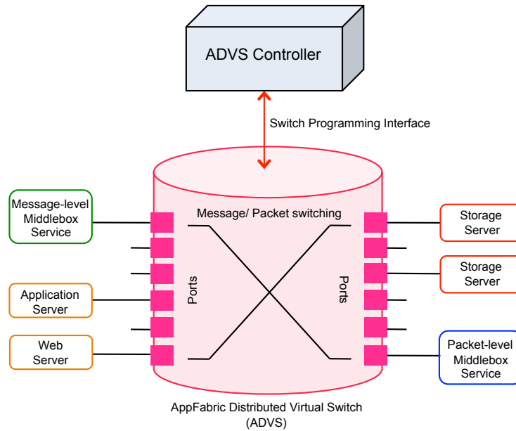
Figure 6.8: AppFabric Distributed Virtual Switch (reproduction of Fig. 3.4)
