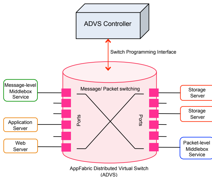
Figure 3.4: AppFabric Distributed Virtual Switch
