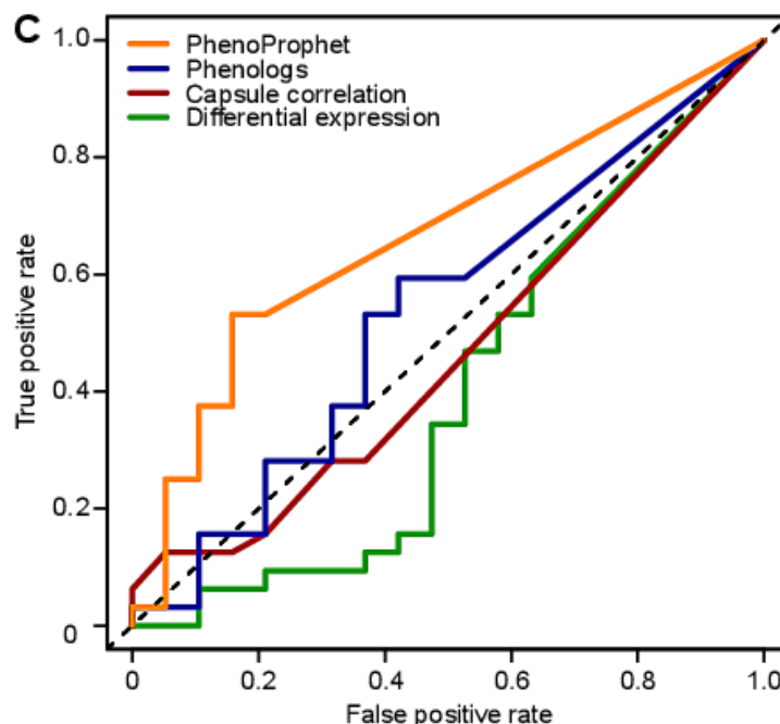
Figure 3.4.C. Receiver operating characteristic analysis comparing the indicated methods for phenotype prediction to random expectation (dotted line).
