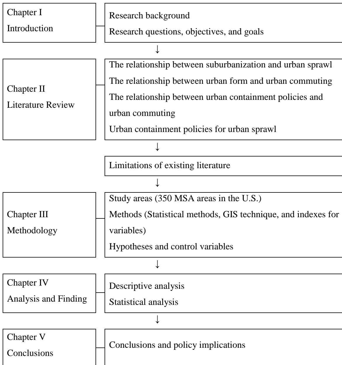
Figure 1. Research Organization
