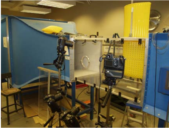
(a) Nylon wing in tunnel.
