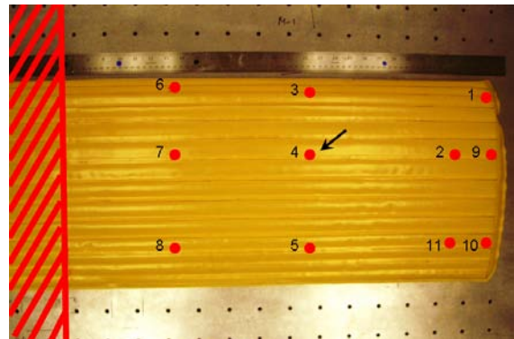
(b) Hammer impulse locations (1-11) and measurement locations (9, 10).
