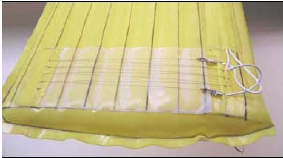
Figure 5.24: SMA wires integrated to an inflatable wing.
