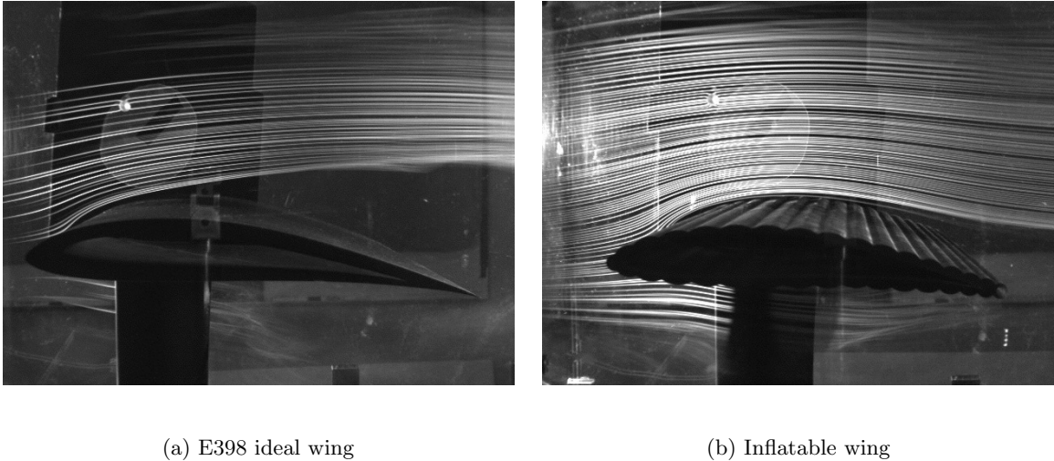
Figure 3.11: Re = 50,000 ; \alpha = 4^\circ [21].
