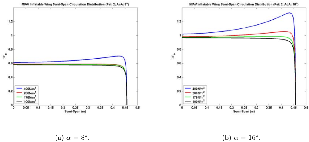
Figure 6.14: Nylon Inflatible Wing Semi-Span Circulation Distribution at 13.8 kPa (2 psi).
