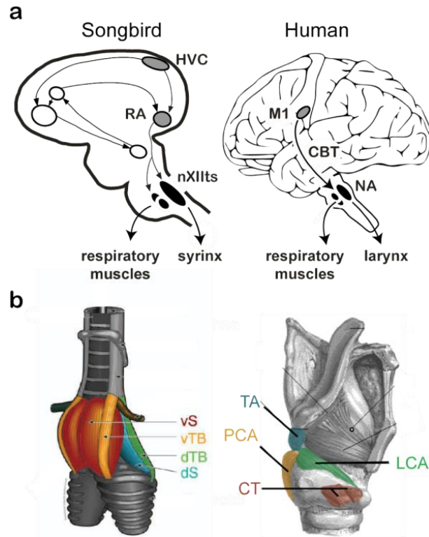
Figure 3: Comparative look at the neural and muscular anatomies of vocalization in humans and songbirds. (a) In songbirds, premotor nucleus RA (robust nucleus of the arcopallium) connects to the 12 th motor nucleus (nXIIts) which innervates the vocal muscles [20, 21, 43]. In humans, the primary motor cortex (M1) projects along the corticobulbar tract (CBT) to the nucleus ambiguus (NA), which innervates the vocal muscles. (b) In songbirds, the dorsal syringeal (DS) and dorsal tracheobronchial (DTB) muscles adduct the vocal membrane, while the ventral tracheo-bronchial (VTB) muscle abducts it. The ventral syringeal (VS) muscle controls membrane tension [44]. In humans, transverse arytenoid (TA) and lateral cricoarytenoid (LCA) adducts the vocal membrane, while the posterior cricoarytenoid (PCA) abducts it. The cricothyroid (CT) muscles control membrane tension. Figure designed by Sam Sober and adapted from [44].
