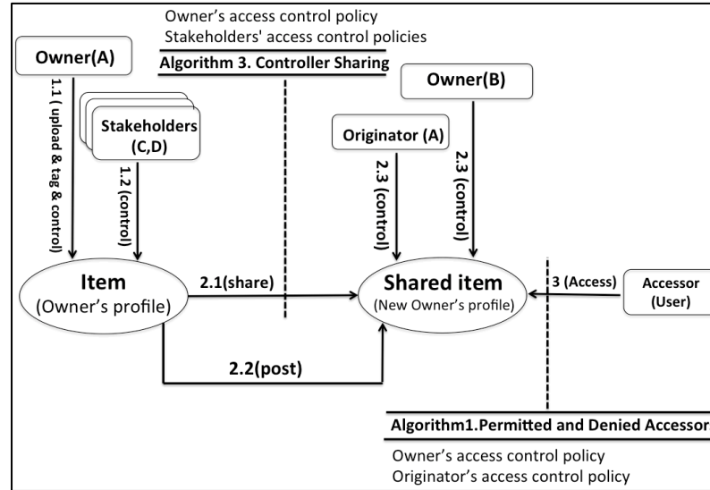
Figure 8: Tagging-sharing users' contents with other user scenario.
