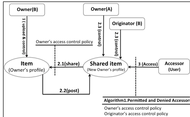
Figure 10: Simple sharing others users' contents scenario.
