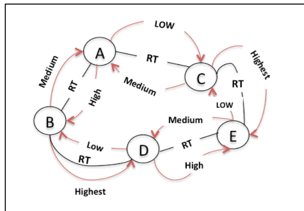
Figure 18: Trust Graph.
