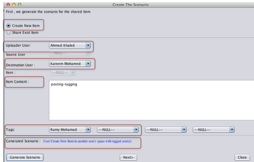
Figure 26: Posting-Tagging scenario.
