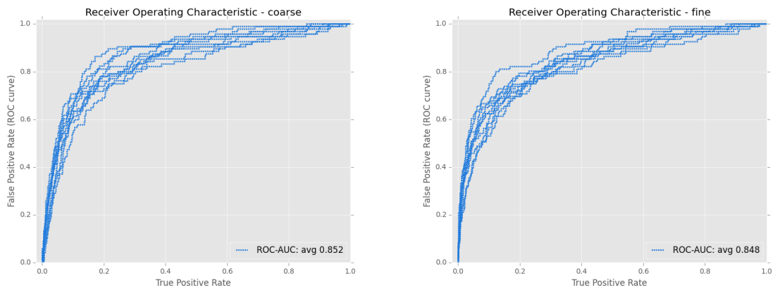
(a) Coarse ROC curves at Round 20
