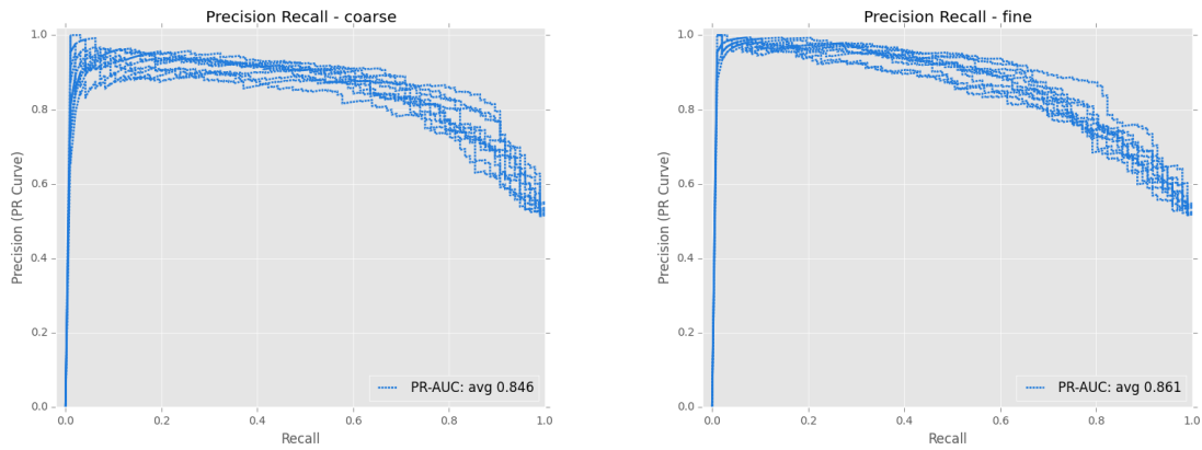
(a) Coarse PR curves at Round 20
