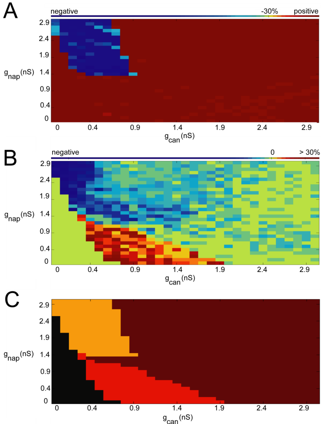
Figure 5.6 Different pacemaking modes within the parameter space: NAP-burster & CAN-burster. Within the parameter space of (g_{\text{nap}}, g_{\text{can}}) = (0 \sim 3, 0 \sim 3 \text{ nS}) , Panel A shows the degree of period modulation from depolarizing current injection. Panel B shows the degree of median burst duration modulation in response to depolarizing current injection. Panel C shows the overall results of pacemaking mode identification in the parameter space. The lower-left corner (black) in Panel C represents non-pacemakers. The upper-right corner (brown) in the same panel represents pacemaking model neurons that
