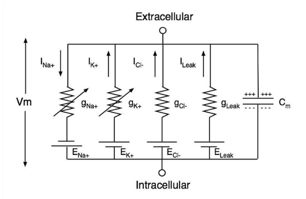
Figure 2.2 A typical action potential and the electrical circuitry representation of a Hodgkin Huxley style neuron model. Panel A illustrates the all-or-non nature of an action potential; the figure is adopted from http://mindoutpsyde.com/forums/index.php?topic=144 . Panel B illustrates the components of a typical Hodgkin-Huxley style model showing how membrane voltage is determined as the electrical potential difference across the cell membrane; this figure is adopted from http://en.wikipedia.org/wiki/File:MembraneCircuit.jpg . The lipid bi-layer cell membrane is represented as a capacitance, and the voltage-gated sodium & potassium channels are represented by time-dependent and
