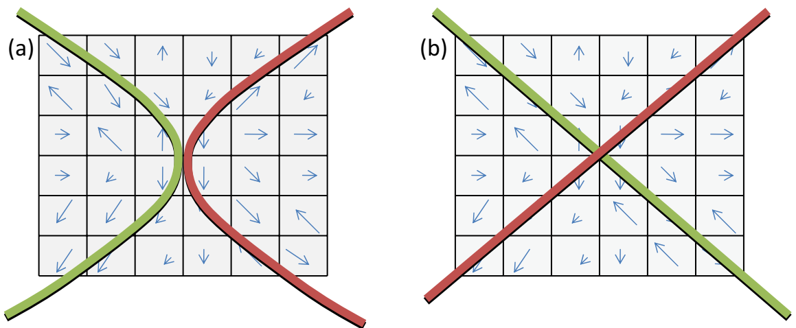
Figure 7: Limitation of DTI: (a) Crossing and (b) Kissing Fibers. The tensor estimation for both the cases is identical and fiber tracking algorithms cannot differentiate between the two.
