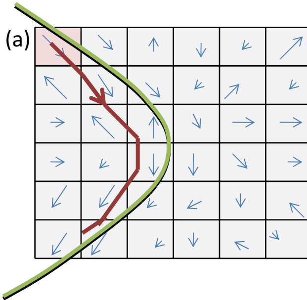
Figure 6: Simple Line Propagation: The green fiber represents the actual fiber arrangement while the fiber in red is traced by using simple line propagation technique. Voxel-by-voxel tensor orientation is shown in the background.
