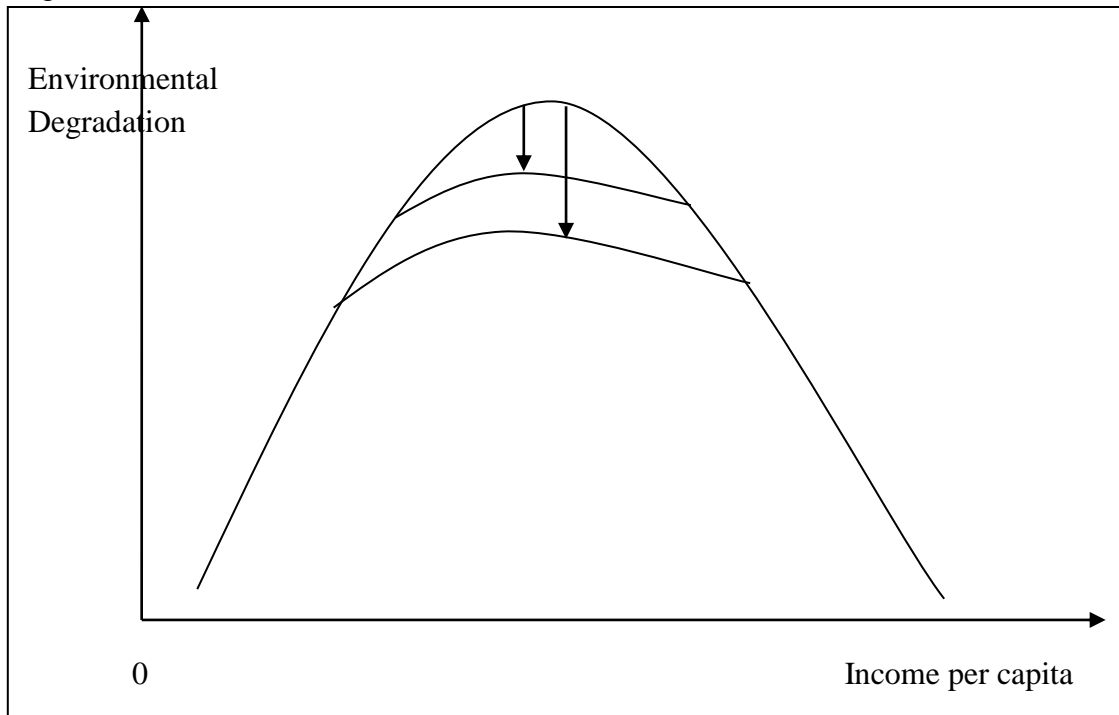
Figure 3.2: Flatter EKC
