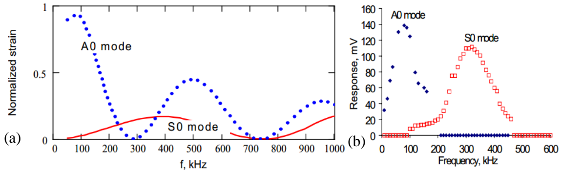
Figure 2.15: (a) Strain Lamb wave tuning results from analytical solution; (b) Experimental results from PWAS response[31].
