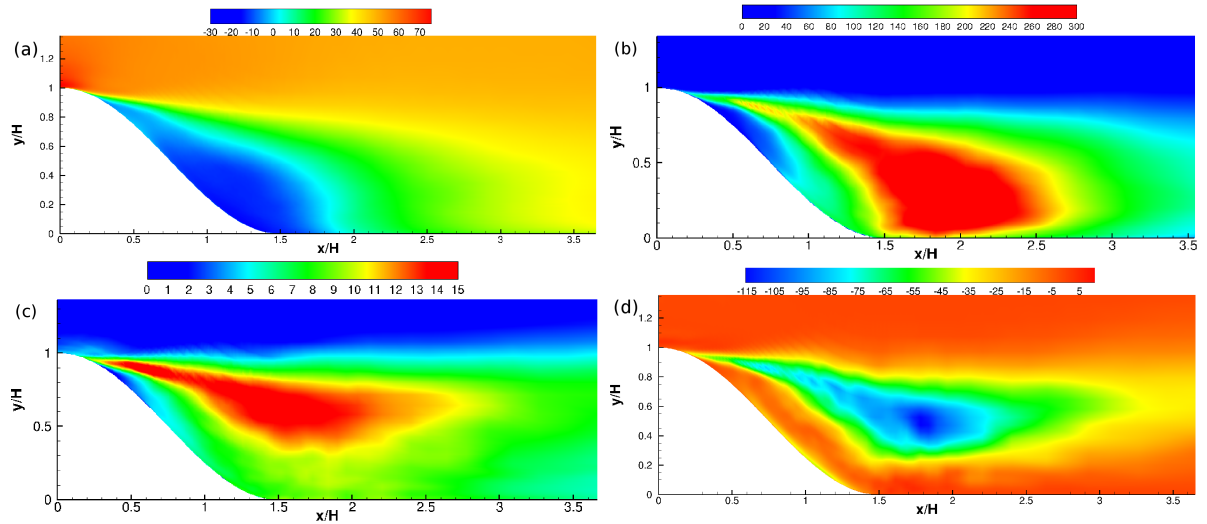
Figure 4.14: Contours of (a) mean streamwise velocity \bar{U} , (b) total turbulent kinetic energy k , (c) u_{rms} , and (d) \overline{u'v'} in the z/H = 0 plane behind the hill
