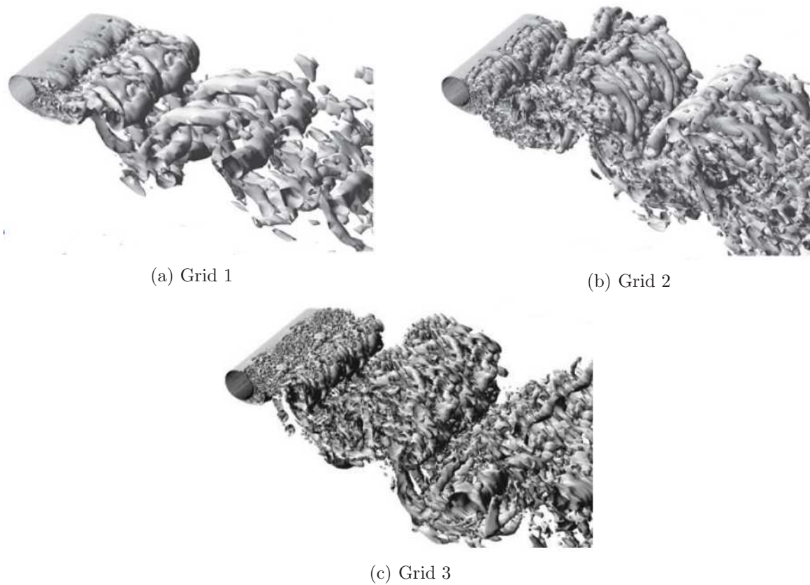
Figure 1.2: Flow over a circular cylinder using the SA-DES model for 3 different grids. Figure reproduced from Spalart (2009).
