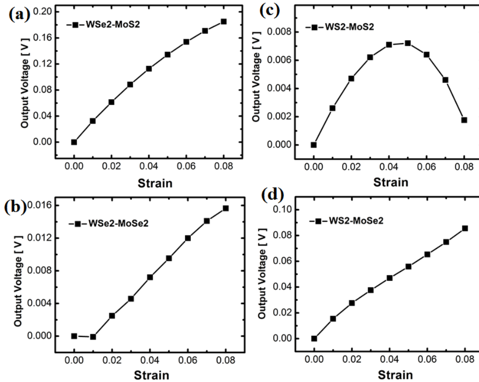
Figure 3.9 The output voltage as a function of strain for 4 heterojunction structures: (a) \text{WSe}_2\text{-MoS}_2 (b) \text{WSe}_2\text{-MoSe}_2 (c) \text{WS}_2\text{-MoS}_2 (d) \text{WS}_2\text{-MoSe}_2
