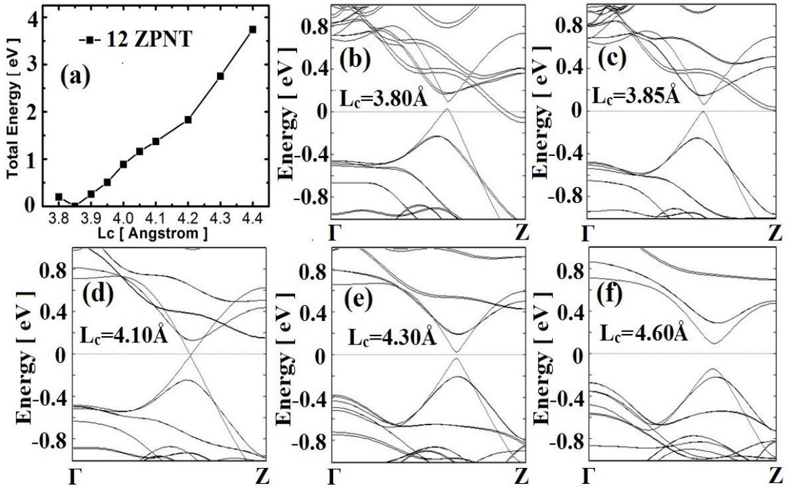
Figure 4.7 (a) the total energy vs. L_c for 12-ZPNT. The bandstructure of 12-ZPNT at (b) L_c = 3.80\text{\AA} ; (c) L_c = 3.85\text{\AA} ; (d) L_c = 4.10\text{\AA} ; (e) L_c = 4.30\text{\AA} ; (f) L_c = 4.60\text{\AA} , respectively. The Fermi level is set to energy=0.
