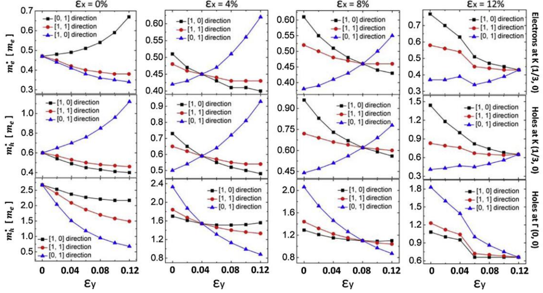
Figure 2.3 The effective mass of charge carriers as the function of strain strength \epsilon_x and \epsilon_y for (a) electrons at K ( 1/3, 0 ), (b) holes at K ( 1/3, 0 ) and (c) holes at \Gamma ( 0, 0 ).
