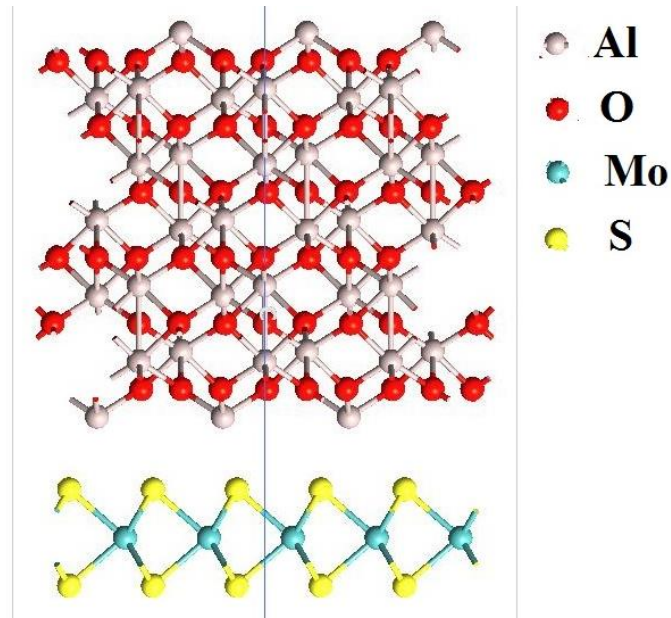
Figure 5.1 Schematic of interface between Al 2 O 3 with MoS 2 monolayer
