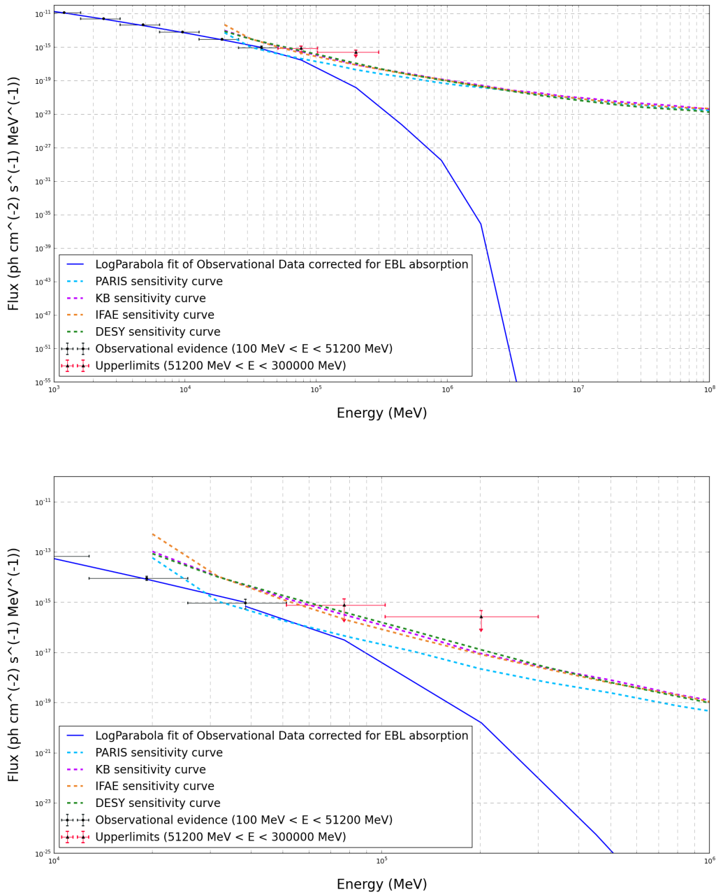
Figure 53: Spectrum of PKS1502+106 for 5-year Fermi analysis together with 50-hour PROD1 sensitivity curves. PKS1502+106 is the third source in order of descending brightness. Contrary to PKS1510-089, our analysis suggests that CTA is unlikely to detect this source with any of the PROD1 analyses considered. Although the PARIS curve is slightly below the spectrum, it does not seem probable that PKS1502+106 will be detected given our criteria and analysis features.
