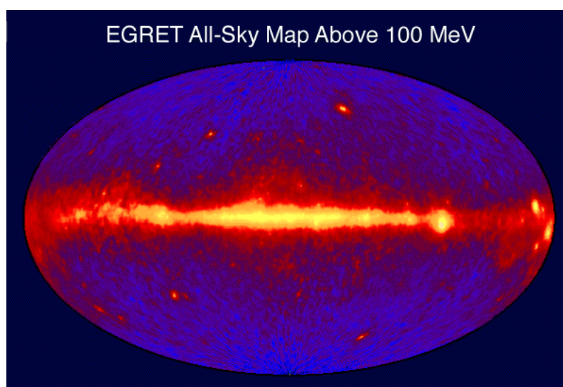
Figure 26: All-sky image from EGRET. Credit: EGRET team.
