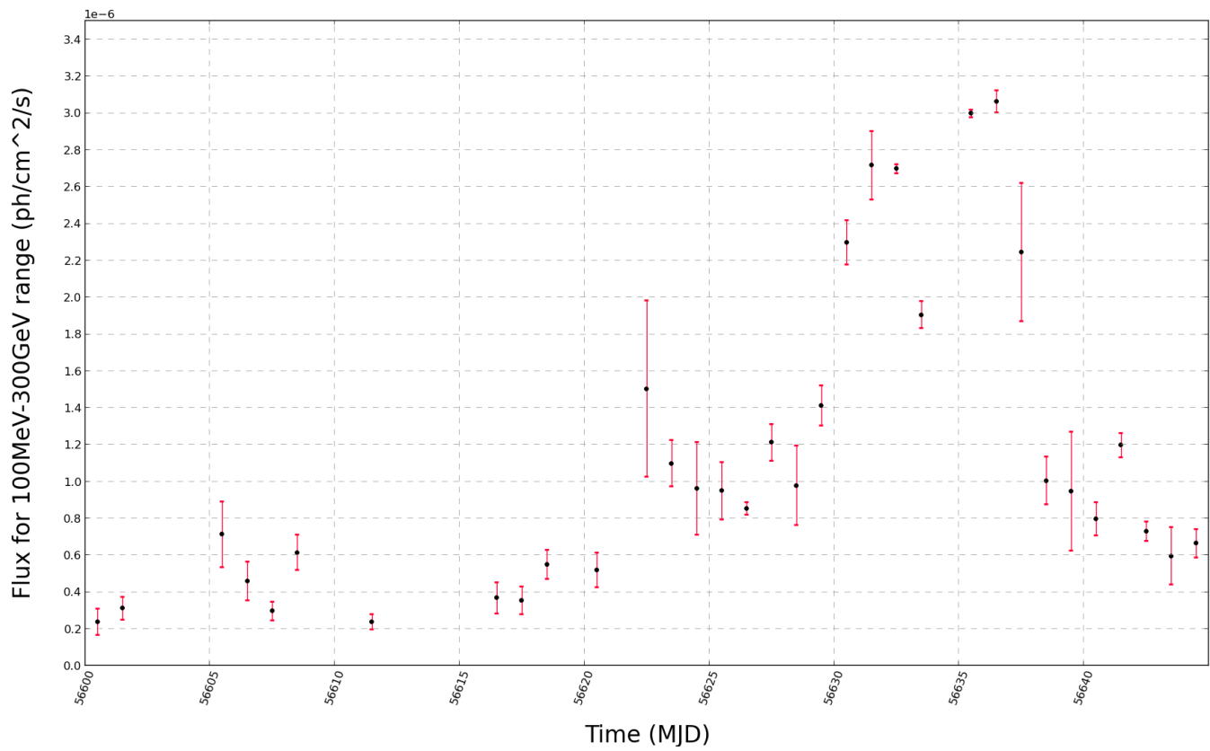
Figure 71: Daily binned light curve for source 3C279.
