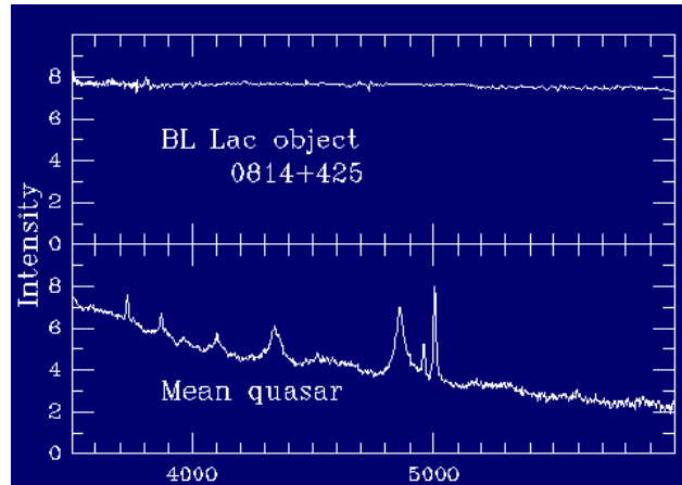
Figure 15: Spectra of a BL Lac object (above) and a mean quasar (below). When compared to the quasar’s, the spectra of the BL Lac object is outstandingly flat. For the “mean quasar” spectrum see Francis et al. 1991, and Lawrence et al. 1996 for 0814+425.
