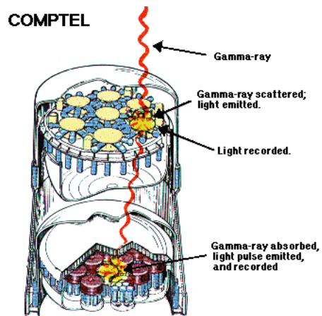
Figure 23: Sketch of the Compton scatter telescope on board NASA's Compton Gamma-Ray Observatory. Image credit: NASA.
