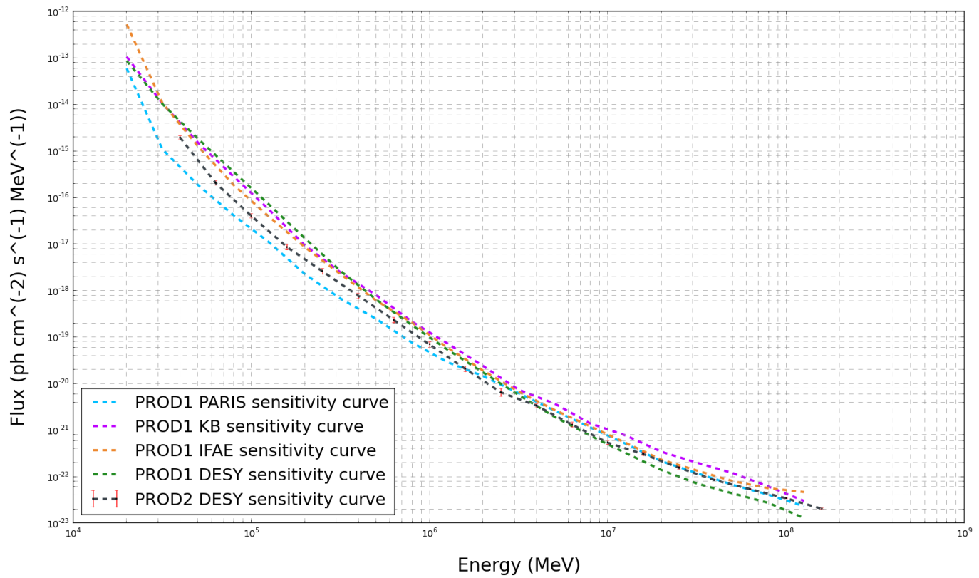
Figure 40: Plot of sensitivity curves considered for long-term analysis (PROD1) and for flare event analysis (PROD2).
