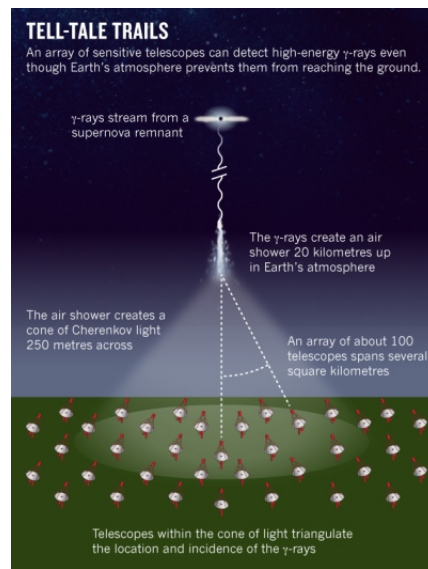
Figure 32: Schematic detection of a gamma-ray coming from a source, a supernovae remnant concretely. The Cherenkov light pool is detected by the telescopes located both totally and partially inside the light cone. Image credit: Eugenie Samuel Reich.
