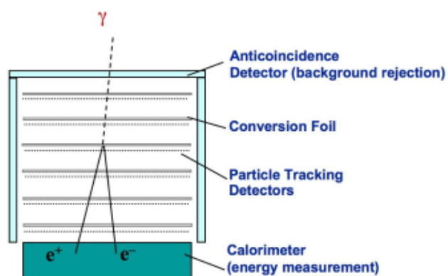
Figure 28: A sketch showing the subsystems composing the LAT instrument aboard the Fermi Gamma-Ray Space Telescope. Image credit: Fermi collaboration.
