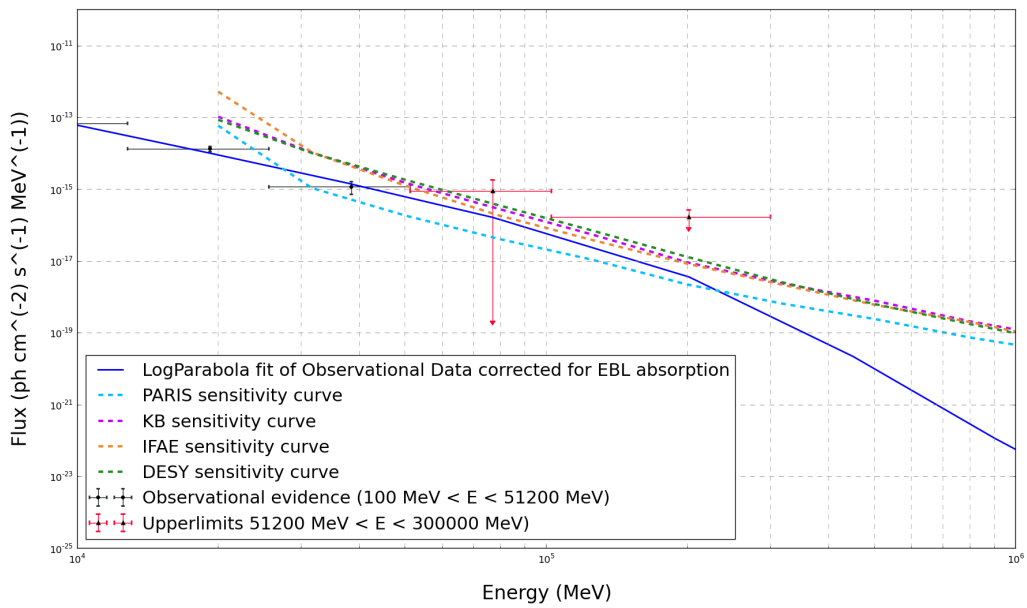
Figure 55: Spectrum of 3C279 for 5-year Fermi analysis together with 50-hour PROD1 sensitivity curves. 3C279 is the fifth source in our list, and according to our analysis, only the PROD1 PARIS analysis would be able to detect it.
