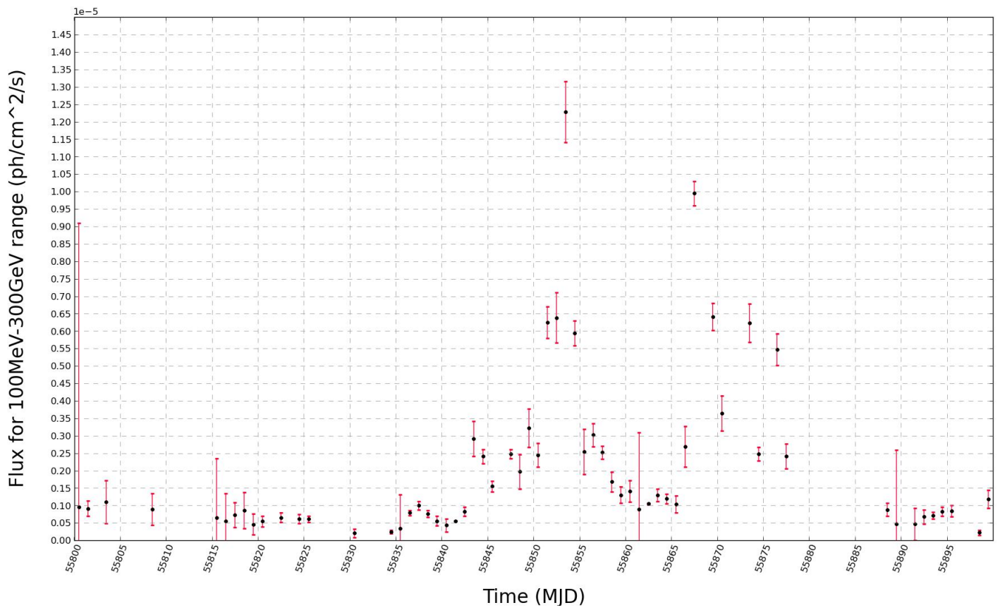
Figure 68: Daily binned light curve for source PKS1510-089.
