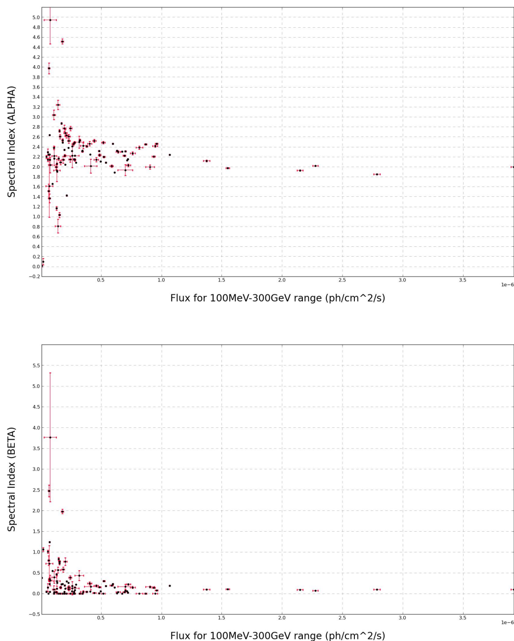
Figure 75: Spectral indexes versus flux for source 4C+21.35 . ABOVE - \alpha vs flux. BELOW - \beta vs flux. No correlation between flux and spectral index is found. Low flux values present larger error bars possibly due to low statistics in this range, resulting in low TS values (and hence significance) of these events.
