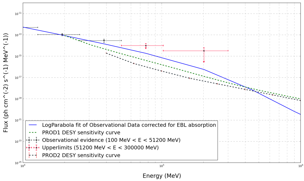
Figure 85: Plot of the spectrum for the brightest flare of 4C+21.35 together with 5-hour PROD1 and PROD2 DESY sensitivity curves. For the 4th source considered for flare analysis, the two configurations considered would enable CTA to observe this FSRQ.
