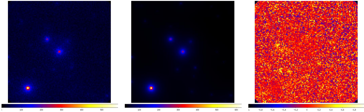
Figure 49: Source 3C273. LEFT - 100 MeV-300 GeV map for the whole 5 year period. Counts per pixel are shown on the color bar. The image scale is 0.2^\circ per pixel, and the image covers 22^\circ \times 22^\circ . CENTER - Model map obtained with the gtmodel Fermi tool for the whole 5 year period, using the best fit model which for 3C273 is a LogParabola. Counts per pixel are shown on the color bar. The image scale is 0.2^\circ per pixel, and the image covers 22^\circ \times 22^\circ . RIGHT - Residuals map of the 100 MeV-300 GeV events in units of percentage. The residuals map is produced by (\text{sky map} - \text{model map})/(\text{model map}) . The colour scales for both the sky map and the model map are in units of gamma-ray counts, whereas the residuals maps are in units of percentage. No evidence is visible for new gamma-ray sources.
