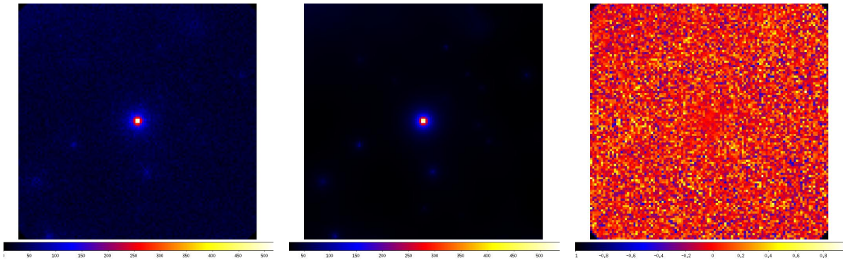
Figure 46: Source PKS0454-234. LEFT - 100 MeV-300 GeV map for the whole 5 year period. Counts per pixel are shown on the color bar. The image scale is 0.2^\circ per pixel, and the image covers 22^\circ \times 22^\circ . CENTER - Model map obtained with the gtmodel Fermi tool for the whole 5 year period, using the best fit model which for PKS0454-234 is a LogParabola. Counts per pixel are shown on the color bar. The image scale is 0.2^\circ per pixel, and the image covers 22^\circ \times 22^\circ . RIGHT - Residuals map of the 100 MeV-300 GeV events in units of percentage. The residuals map is produced by (\text{sky map} - \text{model map})/(\text{model map}) . The colour scales for both the sky map and the model map are in units of gamma-ray counts, whereas the residuals maps are in units of percentage. No evidence is visible for new gamma-ray sources.
