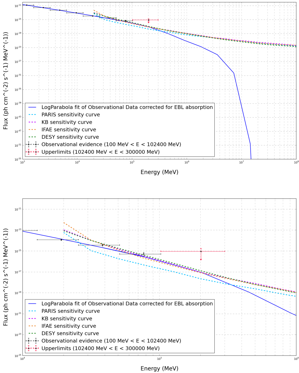
Figure 54: Spectrum of 4C+21.35 for 5-year Fermi analysis together with 50-hour PROD1 sensitivity curves. For the 5-years' worth of data we have considered, the configuration of the PROD1 PARIS sensitivity curve would represent a positive detection of the FSRQ 4C+21.35. For the remaining 3 PROD1 analyses, it is unlikely that the object will be detected, although the sensitivity of the PROD1 IFAE curve is a bit below the spectrum.
