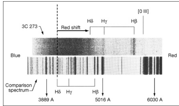
Figure 11: Optical spectrum of the distant quasar 3C273 (redshift z=0.158 ). The redshift of the hydrogen spectral lines H\delta , H\gamma and H\beta is clearly visible. The large redshift indicates how distant the source is, and the width of the lines points towards rapid internal motion within the quasar itself. Image credit: Palomar/Caltech.
