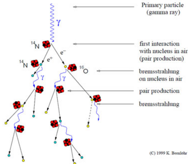
Figure 30: Scheme of a gamma-ray shower originated by the photon interacting with the molecules from the Earth's atmosphere. Image credit: K. Bernlohr.
