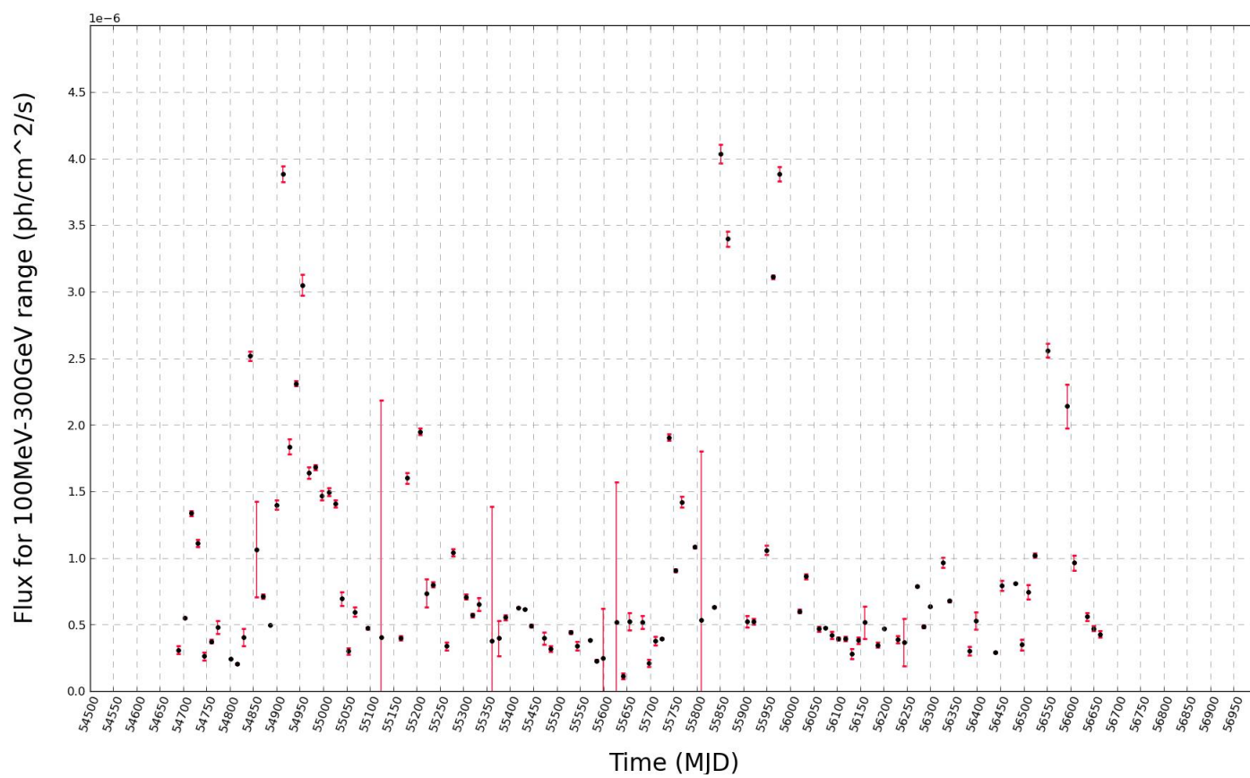
Figure 63: 2-weekly binned light curve for source PKS1510-089.
