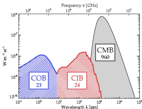
Figure 17: Illustration of the intensity of the EBL. The CMB is also shown to compare the different wavelengths corresponding to each background radiation. The two components of the EBL, the COB and the CIB are clearly distinguishable. The brightness of each component is written in boxes (in units of nW/m^2/sr ). From Dole et al., 2006.
