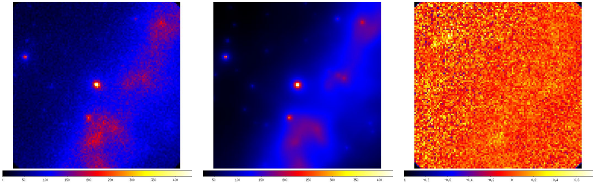
Figure 47: Source PKS0727-11. LEFT - 100 MeV-300 GeV map for the whole 5 year period. Counts per pixel are shown on the color bar. The image scale is 0.2^\circ per pixel, and the image covers 22^\circ \times 22^\circ . CENTER - Model map obtained with the gtmodel Fermi tool for the whole 5 year period, using the best fit model which for PKS0727-11 is a LogParabola. Counts per pixel are shown on the color bar. The image scale is 0.2^\circ per pixel, and the image covers 22^\circ \times 22^\circ . RIGHT - Residuals map of the 100 MeV-300 GeV events in units of percentage. The residuals map is produced by (\text{sky map} - \text{model map})/(\text{model map}) . The colour scales for both the sky map and the model map are in units of gamma-ray counts, whereas the residuals maps are in units of percentage. No evidence is visible for new gamma-ray sources.
