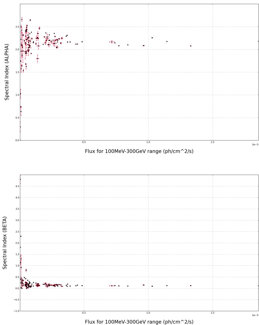
Figure 72: Spectral indexes versus flux for source 3C454.3. ABOVE - \alpha vs flux. BELOW - \beta vs flux. No correlation between flux and spectral index is found. Low flux values present larger error bars possibly due to low statistics in this range, resulting in low TS values (and hence significance) of these events.
