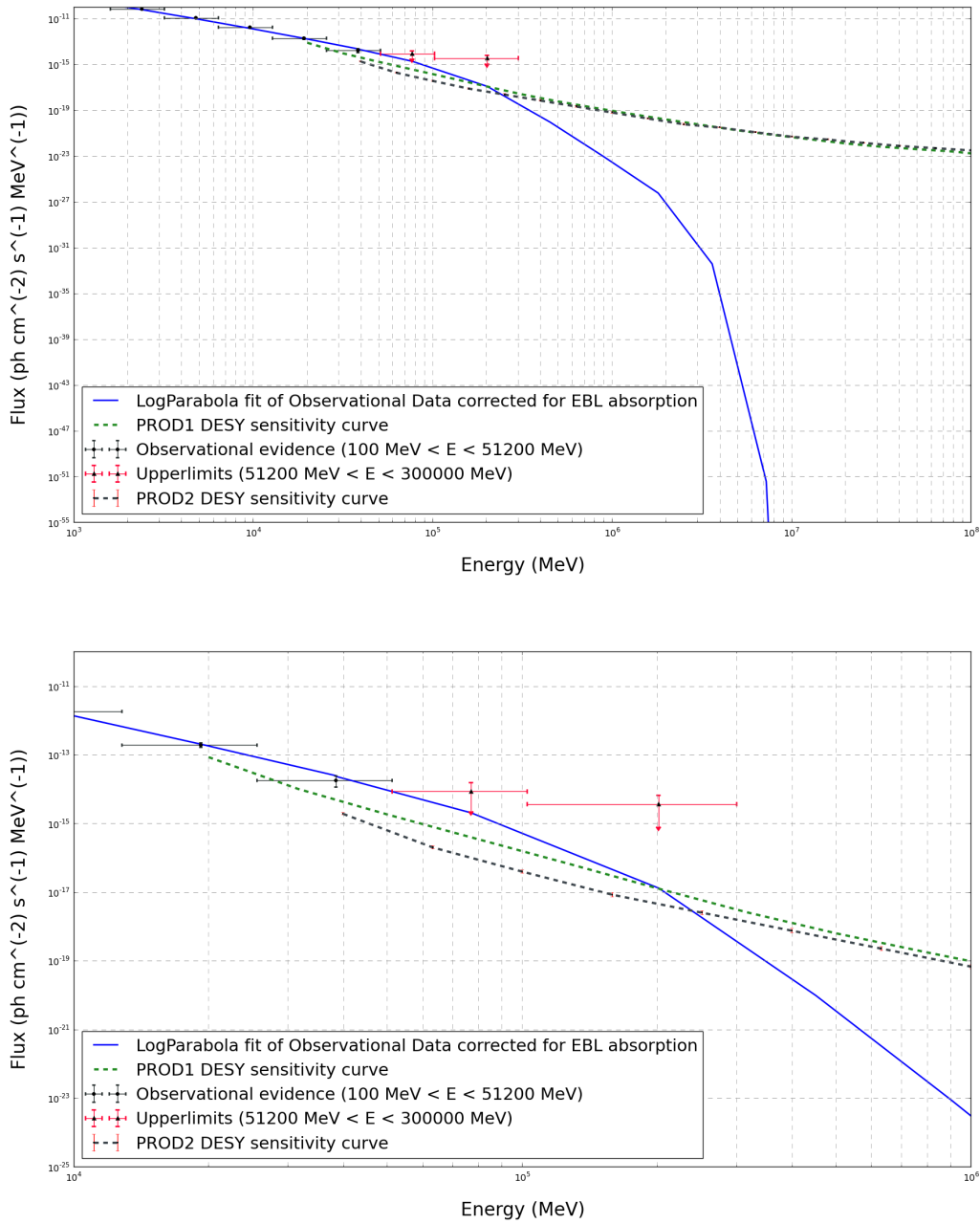
Figure 82: Plot of the spectrum for the brightest flare of 3C454.3 together with 5-hour PROD1 and PROD2 DESY sensitivity curves. The shape of the spectra during the flare and for the 5-year analysis are quite similar: the EBL absorption reduces the observed flux drastically for energies above 10 5 MeV. The lower plot illustrates that the PROD2 DESY configuration is more sensitive than the PROD1 DESY configuration, even if the latter extends to lower energies. But it is more interesting to obtain a better sensitivity for higher energies, since this is where the difficulty for detecting FSRQs rises. Nonetheless, for the FSRQ 3C454.3, both configurations would enable the detection the source according to this analysis.
