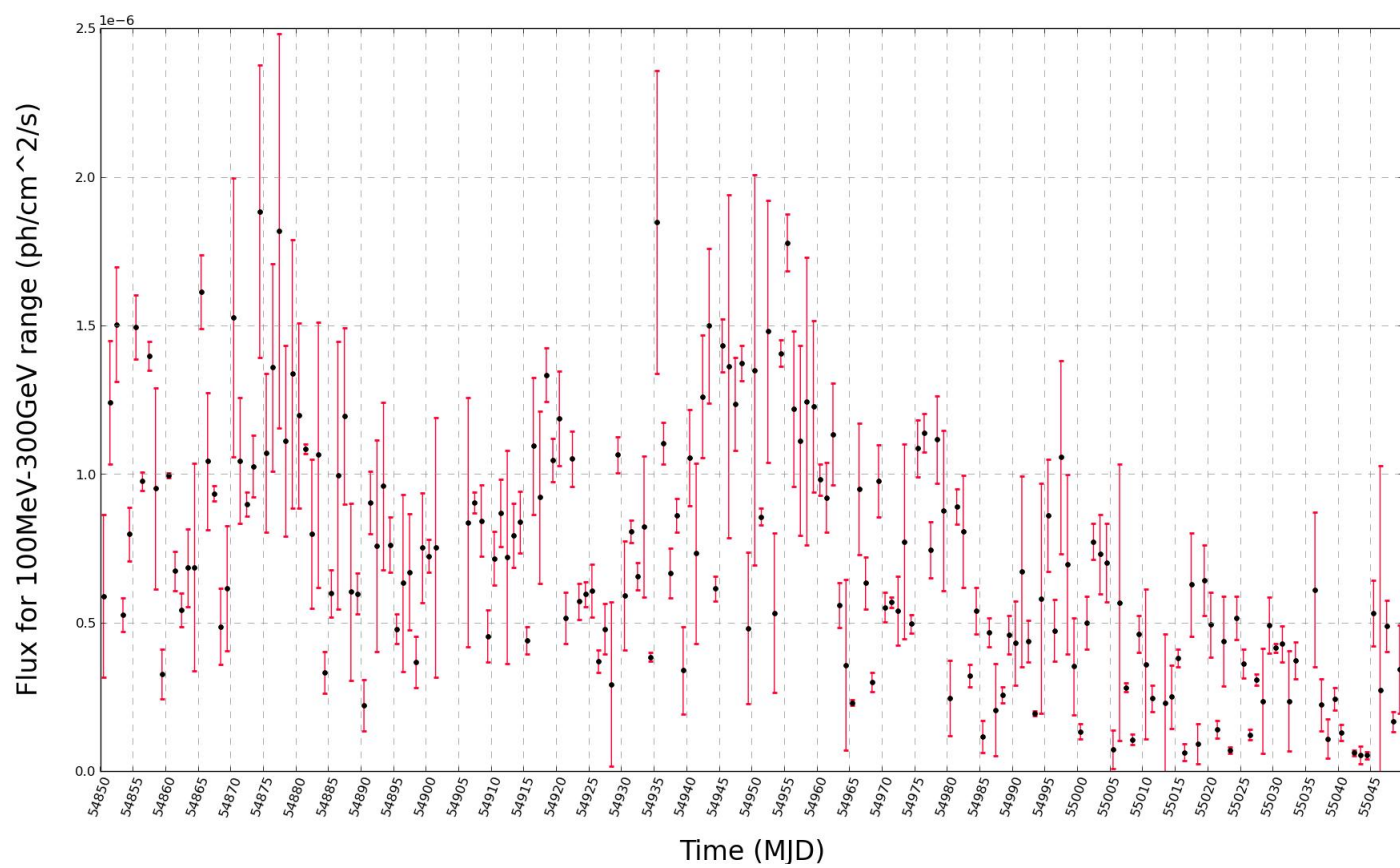
Figure 69: Daily binned light curve for source PKS1502+106.
