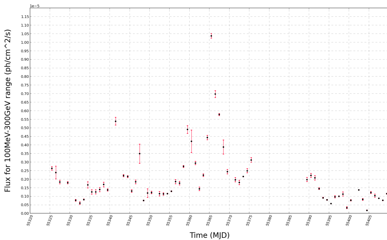
Figure 70: Daily binned light curve for source 4C+21.35.
