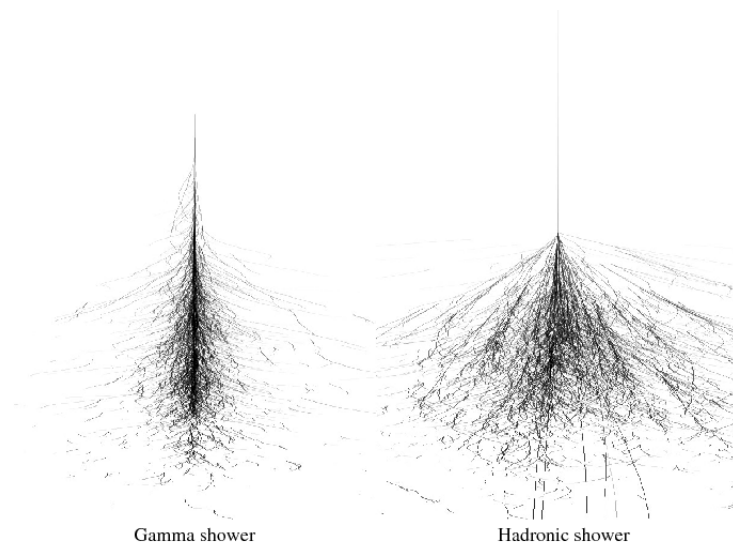
Figure 31: Imaging of a gamma-ray induced particle cascade (left) and cosmic-ray induced shower (right). Gamma-rays create narrower showers that are more aligned with the direction of the incoming photon [69].
