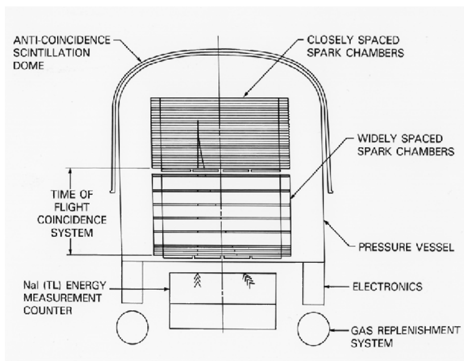
Figure 25: Scheme of the pair detector used in EGRET (Energetic Gamma-Ray Experiment Telescope). The anticoincidence detector, the spark chamber and the calorimeter used for detecting clean events can be clearly seen in the diagram. Image credit goes to CGRO Science Support Centre.
