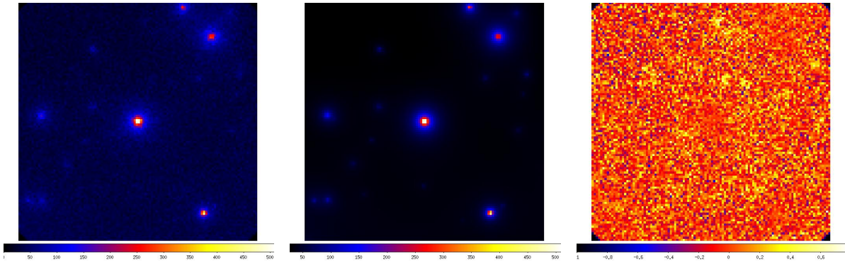
Figure 45: Source 3C279. LEFT - 100 MeV-300 GeV map for the whole 5 year period. Counts per pixel are shown on the color bar. The image scale is 0.2^\circ per pixel, and the image covers 22^\circ \times 22^\circ . CENTER - Model map obtained with the gtmodel Fermi tool for the whole 5 year period, using the best fit model which for 3C2793 is a LogParabola. Counts per pixel are shown on the color bar. The image scale is 0.2^\circ per pixel, and the image covers 22^\circ \times 22^\circ . RIGHT - Residuals map of the 100 MeV-300 GeV events in units of percentage. The residuals map is produced by (\text{sky map} - \text{model map})/(\text{model map}) . The colour scales for both the sky map and the model map are in units of gamma-ray counts, whereas the residuals maps are in units of percentage. No evidence is visible for new gamma-ray sources.
