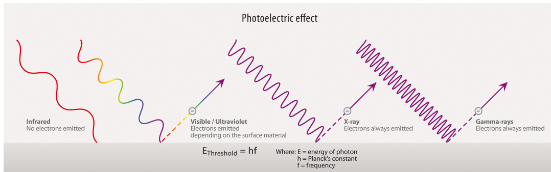
Figure 1: Illustration of the photoelectric effect [60].
