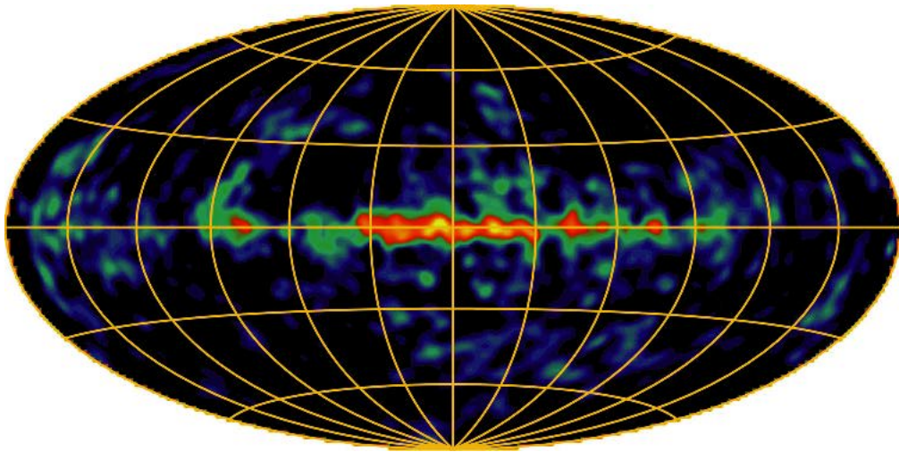
Figure 24: All-sky map from Comptel. The poor angular resolution is clearly noticeable. Image credit: Comptel collaboration.
