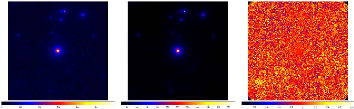
Figure 44: Source 4C+21.35 . LEFT - 100 MeV-300 GeV map for the whole 5 year period. Counts per pixel are shown on the color bar. The image scale is 0.2^\circ per pixel, and the image covers 22^\circ \times 22^\circ . CENTER - Model map obtained with the gtmodel Fermi tool for the whole 5 year period, using the best fit model which for 4C+21.35 is a LogParabola . Counts per pixel are shown on the color bar. The image scale is 0.2^\circ per pixel, and the image covers 22^\circ \times 22^\circ . RIGHT - Residuals map of the 100 MeV-300 GeV events in units of percentage. The residuals map is produced by (\text{sky map} - \text{model map})/(\text{model map}) . The colour scales for both the sky map and the model map are in units of gamma-ray counts, whereas the residuals maps are in units of percentage. No evidence is visible for new gamma-ray sources.
