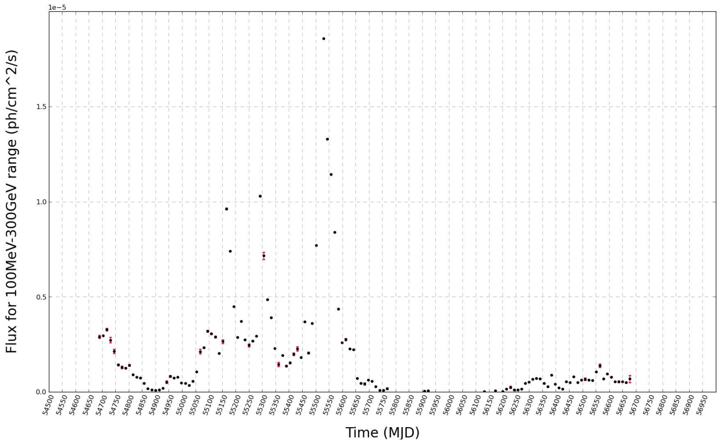
Figure 62: 2-weekly binned light curve for source 3C454.3. Several bright flares are obvious, followed by some periods of time for which the source is not even detected, or very low fluxes are detected.
