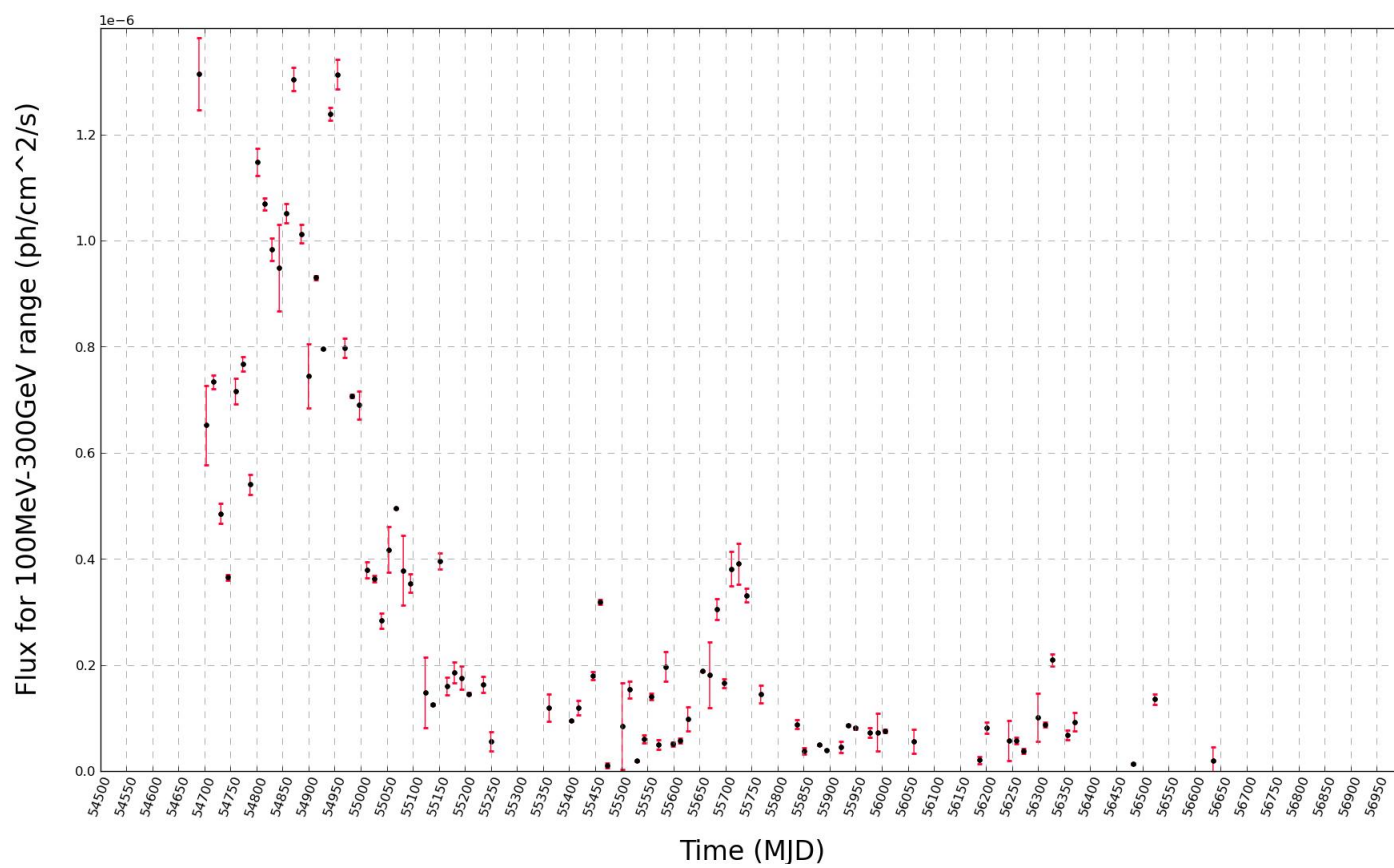
Figure 64: 2-weekly binned light curve for source PKS1502+106.
