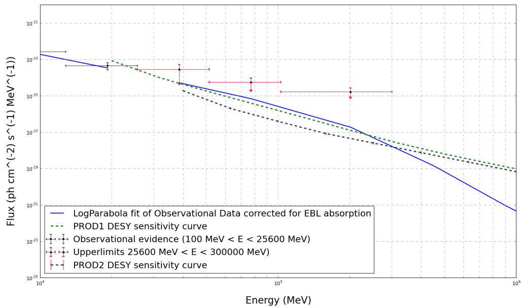
Figure 86: Plot of the spectrum for the brightest flare of 3C279 together with 5-hour PROD1 and PROD2 DESY sensitivity curves. Likewise the rest of the sources analysed during flare intervals, 3C79 would be observed by both PROD1 and PROD2 DESY configurations.
