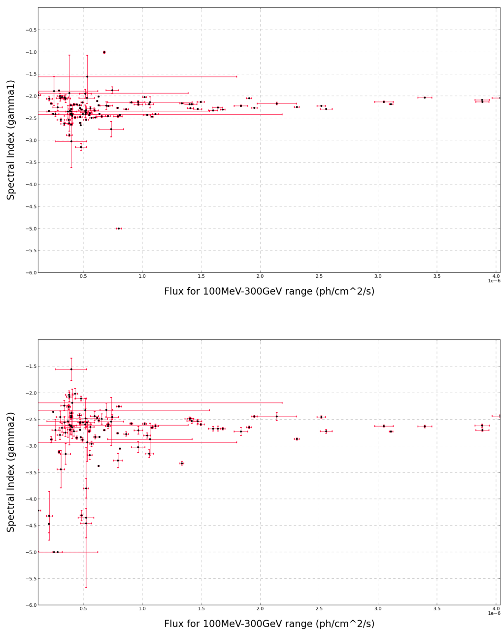
Figure 73: Spectral indexes versus flux for source PKS1510-089. ABOVE - \gamma_1 vs flux. BELOW - \gamma_2 vs flux. No correlation between flux and spectral index is found. Low flux values present larger error bars possibly due to low statistics in this range, resulting in low TS values (and hence significance) of these events.
