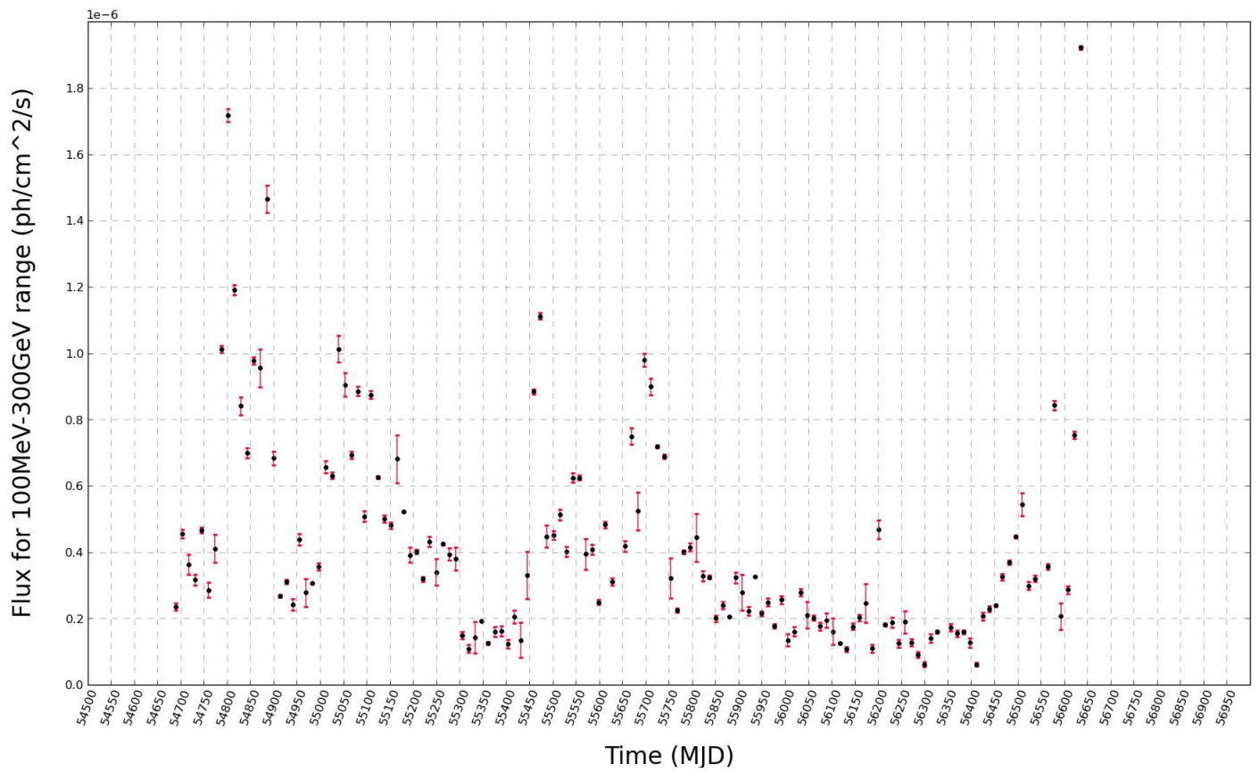
Figure 66: 2-weekly binned light curve for source 3C279.
