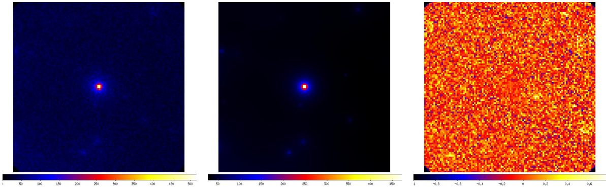
Figure 43: Source PKS1502+106 . LEFT - 100 MeV-300 GeV map for the whole 5 year period. Counts per pixel are shown on the color bar. The image scale is 0.2^\circ per pixel, and the image covers 22^\circ \times 22^\circ . CENTER - Model map obtained with the gtmodel Fermi tool for the whole 5 year period, using the best fit model which for PKS1502+106 is a LogParabola . Counts per pixel are shown on the color bar. The image scale is 0.2^\circ per pixel, and the image covers 22^\circ \times 22^\circ . RIGHT - Residuals map of the 100 MeV-300 GeV events in units of percentage. The residuals map is produced by (\text{sky map} - \text{model map})/(\text{model map}) . The colour scales for both the sky map and the model map are in units of gamma-ray counts, whereas the residuals maps are in units of percentage. No evidence is visible for new gamma-ray sources.
