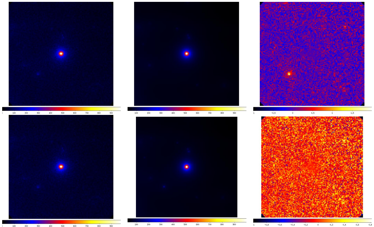
Figure 50: Source 3C273. LEFT COLUMN - 100 MeV-300 GeV map for the whole 5 year period. Counts per pixel are shown on the color bar. The image scale is 0.2^\circ per pixel, and the image covers 22^\circ \times 22^\circ . CENTER COLUMN - Model map obtained with the gtmodel Fermi tool for the whole 5 year period, using the best fit model which for 3C273 is a LogParabola. Counts per pixel are shown on the color bar. The image scale is 0.2^\circ per pixel, and the image covers 22^\circ \times 22^\circ . RIGHT COLUMN - Residuals map of the 100 MeV-300 GeV events in units of percentage. The residuals map is produced by (sky map - model map)/(model map). UPPER ROW - Source PKS1510-089 modelled as a BrokenPowerLaw. LOWER ROW - Source PKS1510-089 modelled as BrokenPowerLaw with point-like source added as a PowerLaw. The colour scales for both the sky map and the model map are in units of gamma-ray counts, whereas the residuals maps are in units of percentage. No evidence is visible for new gamma-ray sources.
