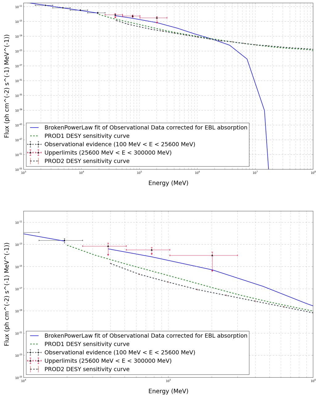
Figure 83: Plot of the spectrum for the brightest flare of PKS1510-089 together with 5-hour PROD1 and PROD2 DESY sensitivity curves. PKS1510-089 would be detected using both PROD1 and PROD2 configurations and DESY analysis up to higher energies than the rest of the sources, due to a combination of the BrokenPowerLaw shape of the distribution and the brightness of the flare.
