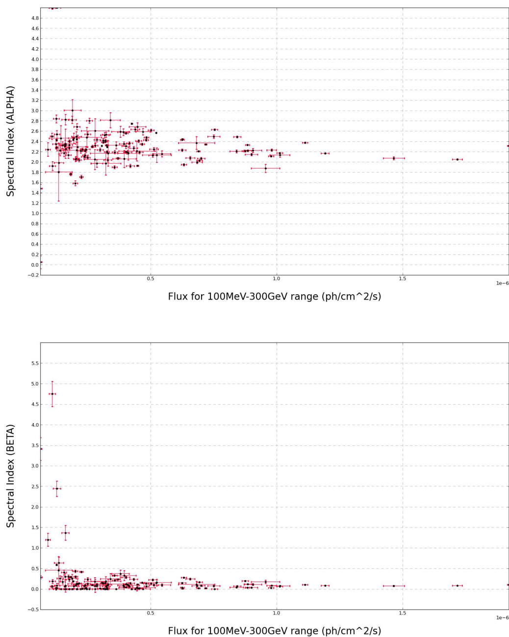
Figure 76: Spectral indexes versus flux for source 3C279. ABOVE - \alpha vs flux. BELOW - \beta vs flux. No correlation between flux and spectral index is found. Low flux values present larger error bars possibly due to low statistics in this range, resulting in TS values (and hence significance) of these events. There is a slight tendency of larger \beta values for lower fluxes, even if there is not an overall correlation.
