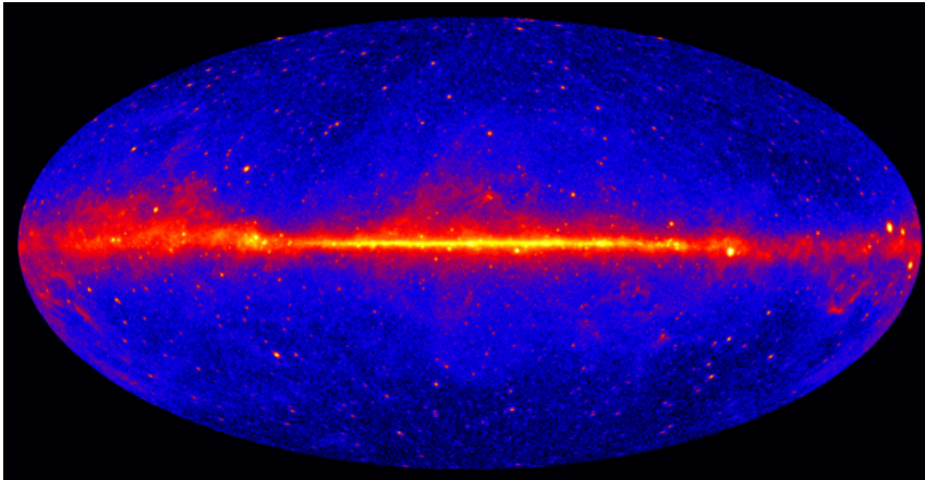
Figure 29: All-sky image constructed from 5 years of observation with Fermi Gamma-Ray Telescope. Brighter colors show brighter gamma-ray sources. The galactic planes is clearly dominating the gamma-ray sky. The majority of AGN detected are located off the plane. Image credit: NASA/DOE/Fermi LAT Collaboration.
