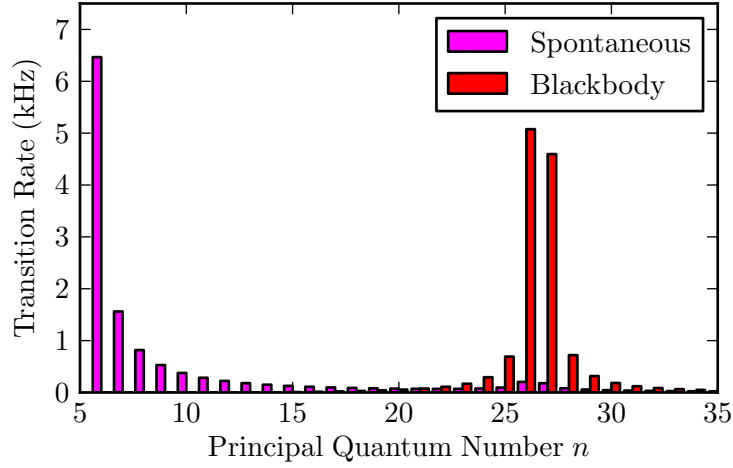
Figure 2.8.: Comparison of spontaneous (blue) and BBR-induced (red) transition rates for 26^2\text{P}_{3/2} \rightarrow n^2\text{S}_{1/2} at temperature T = 350 K.
