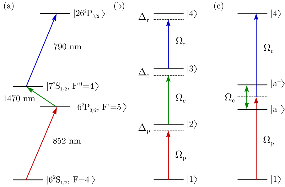
Figure 7.1.: Three-photon excitation scheme to Rydberg states in caesium. (a) Atomic energy level diagram. (b) Bare state energy level diagram. (c) Semi-dressed state energy level diagram where |a^\pm\rangle = (|2\rangle \pm |3\rangle)/\sqrt{2} .
