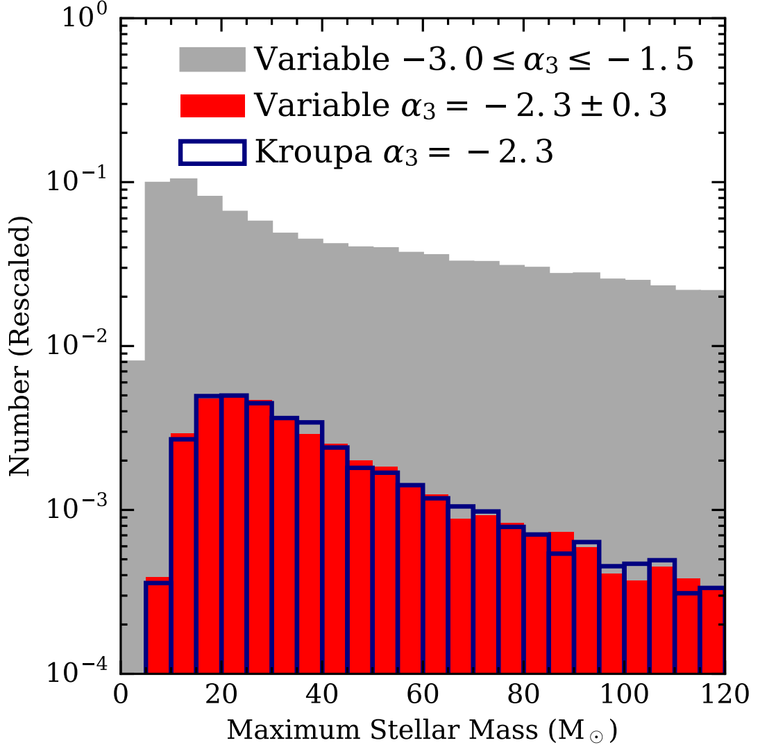
Figure 3.16: Comparison of the maximum stellar mass for two sets of realisations of a 500M_{\odot} cluster at 10^6 yr. In the first set (blue histogram), the stars are drawn from a canonical Kroupa IMF in 5000 realisations. In the second set, we generate 10^5 realisations using the variable IMF mode, with the upper-end slope \alpha_3 drawn from a flat distribution between -3.0 and -1.5 . The subset of realisations with a value of \alpha_3 within \pm 0.3 of the Kroupa value is shown in red, while the full range is shown in grey. The histograms are rescaled such that there are an equal number of clusters in the bins for the Kroupa and constrained variable cases, such that their size is relative to the complete variable set.
