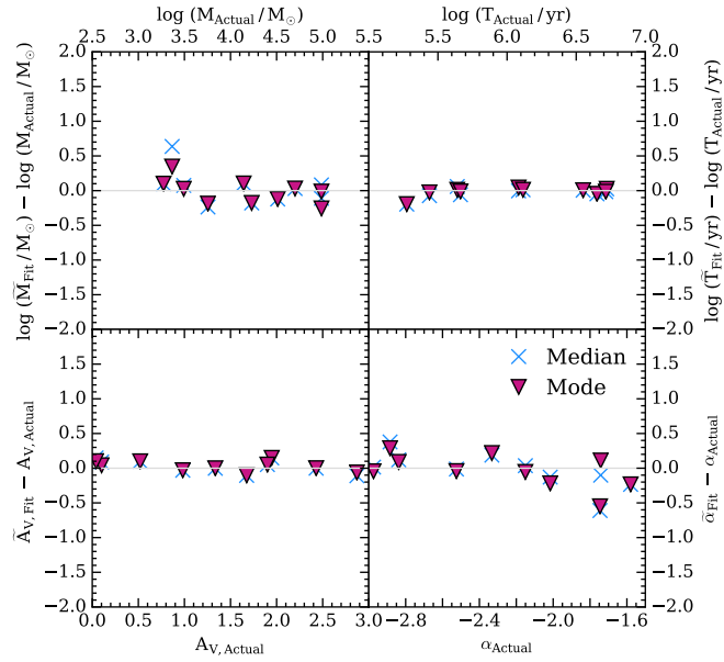
(b) LEGUS filters + lines (CIII, CIVa, NVa, OVa, OV1b )
