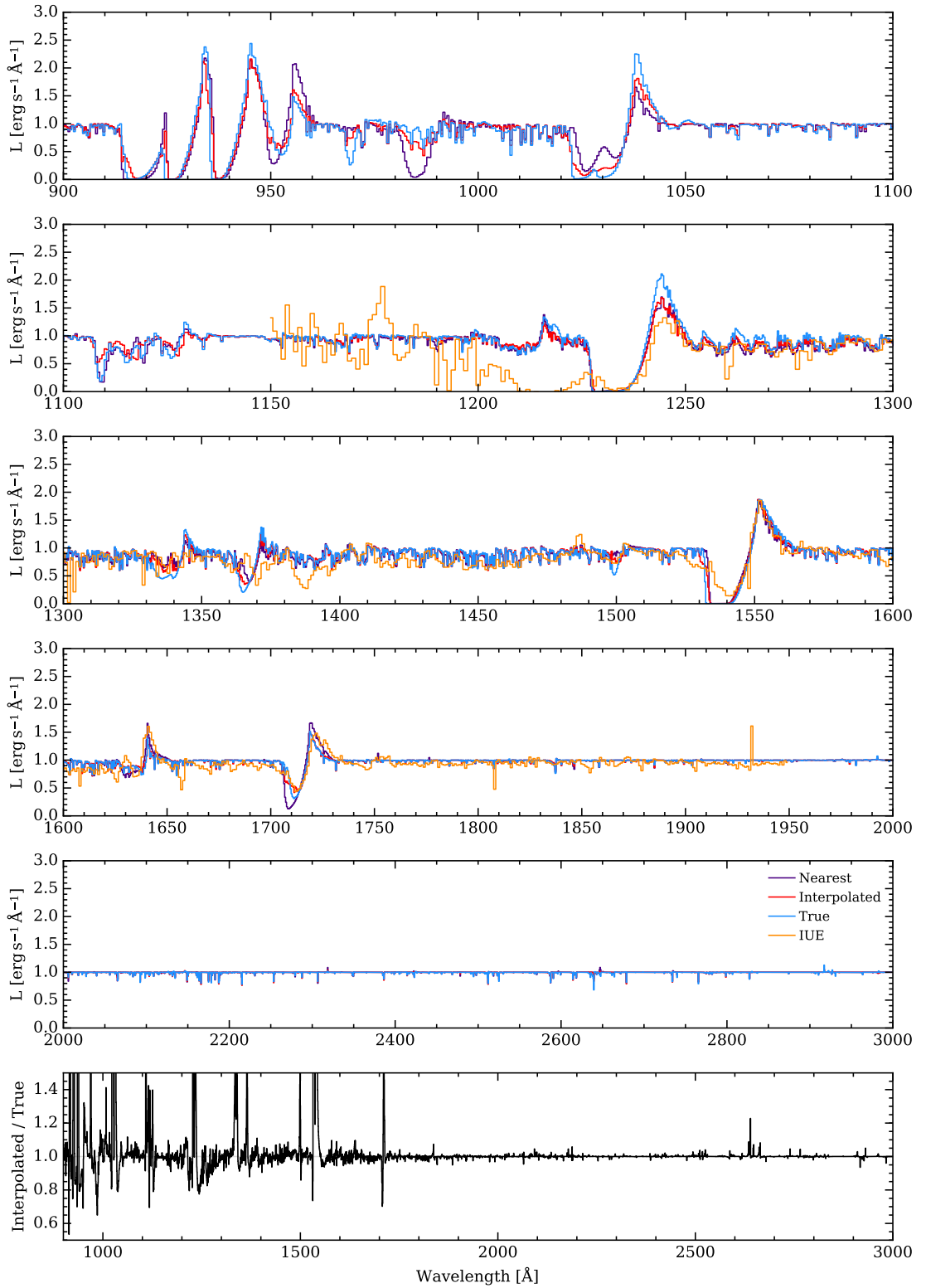
Figure 2.6: Comparison between the spectra for one of the stellar models (model 21) in the IFA atmosphere grid. The true spectrum for that model is plotted in blue. The interpolated spectrum is plotted in red and the nearest neighbour spectrum is plotted in purple, both from an IFA grid with this particular stellar model removed. In orange is shown the observed spectrum for a star of matching type, marked as “IUE” and taken from Walborn et al. (1995a,b) . The observed spectrum is the mean of three O3I spectra from this dataset. For more details on companion stars to model spectra, see Leitherer et al. (2010) .
