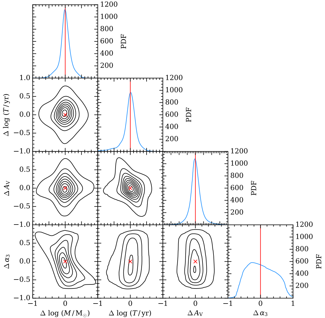
Figure 3.10: Stacks of the one and two-dimensional PDFs (median-centred) for 700 mock clusters simulated with a variable IMF and the choice of parameters listed in Table 3.2. 2D PDF contours are spaced in steps of 100, beginning at 100. The red crosses and lines mark the zero points.
