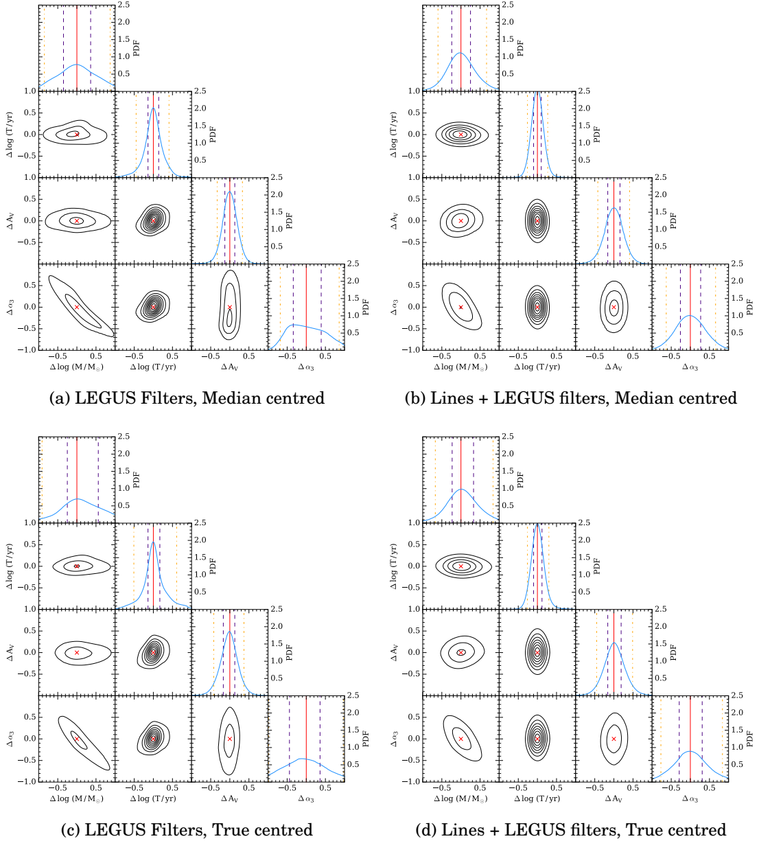
Figure 4.8: Stacks of the one and two-dimensional PDFs for 500 clusters generated as mock observations, as described in Table 4.4. The stacked PDFs are normalised by the number of clusters being stacked, with contours spaced in steps of 0.5, beginning at 0.5. The red crosses and lines mark the zero points. Panels (a) and (c) are the results of analysis using the LEGUS filters only, and are median-centred and centred on the true values respectively. Likewise, panels (b) and (d) show the results of analysis using both the lines (CIII, CIVa, NVa, Ova, OVib) and the LEGUS filters, once again median-centred and true-value-centred respectively. Note the significant improvement in the recovery of the cluster age when including the lines in the analysis. We also see improvement in the recovery of the cluster mass and IMF, although with a residual \log M - \alpha_3 degeneracy in the joint posterior PDF for those parameters. The fifth and ninety-fifth percentiles are marked with orange dot-dashed lines, and the first and third quartiles are marked with indigo dashed lines. The change in the interpercentile ranges (for the true-centred cases, panels (c) and (d)) are given in Table 4.5.
