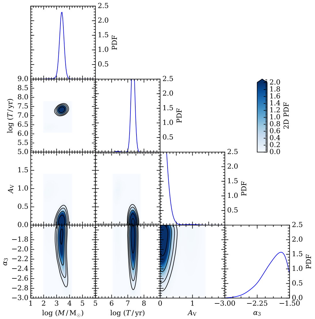
Figure 3.2: As Figure 3.1, but for cluster ID 591.
