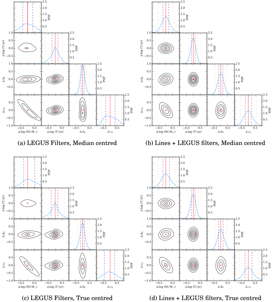
Figure 4.6: Stacks of the one and two-dimensional PDFs for 500 clusters generated as mock observations, as described in Table 4.1. The stacked PDFs are normalised by the number of clusters being stacked, with contours spaced in steps of 0.5, beginning at 0.5. The red crosses and lines mark the zero points. Panels (a) and (c) are the results of analysis using the LEGUS filters only, and are median-centred and centred on the true values respectively. Likewise, panels (b) and (d) show the results of analysis using both the lines (CIII, CIVa, NVa, Ova, OVib) and the LEGUS filters, once again median-centred and true-value-centred respectively. Note the significant improvement in the recovery of the cluster age when including the lines in the analysis. We also see improvement in the recovery of the cluster mass and IMF, although with a residual \log M - \alpha_3 degeneracy in the joint posterior PDF for those parameters. The fifth and ninety-fifth percentiles are marked with orange dot-dashed lines, and the first and third quartiles are marked with indigo dashed lines. The change in the interpercentile ranges (for the true-centred cases, panels (c) and (d)) are given in Table 4.3.
