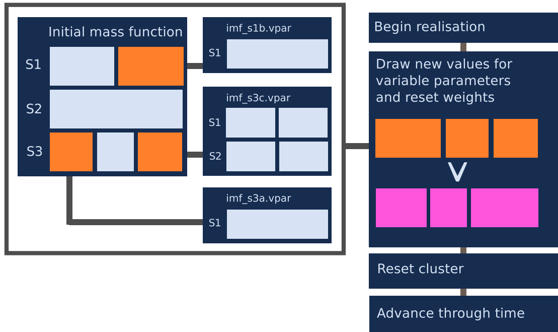
Figure 2.1: A realisation involving a three segment variable IMF, with variable parameters marked in orange. Following through with how SLUG runs, we begin at “begin realisation.” At the start of the realisation we draw new values for the variable parameters and reset the weights on each segment of the PDF containing these variable parameters. The construction of this PDF is shown on the left. In this example, segment one (‘S1’) has its second parameter drawn from a single component PDF. Segment three (‘S3’) on the other hand has its first parameter drawn from a single parameter single segment PDF, and its third parameter drawn from a two segment PDF where each segment has two parameters. The new PDF is displayed in magenta. The code then resets the star cluster and continues with the realisation. This process is then repeated at the next realisation.
