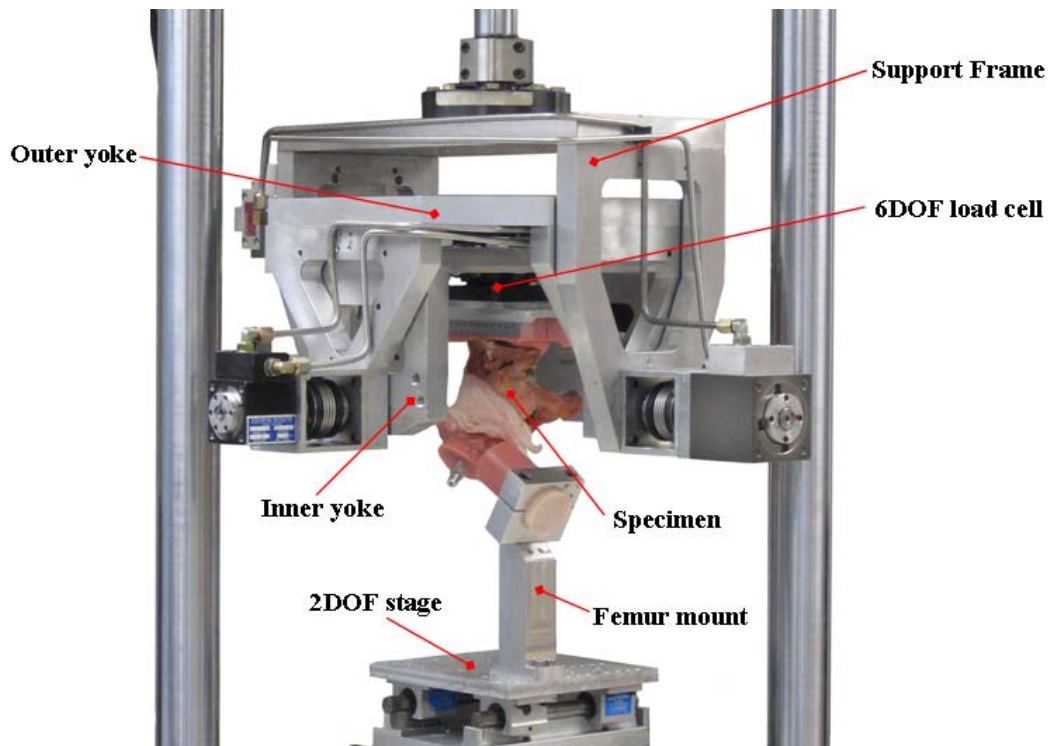
Figure 10. Close-up of the hip simulator.
