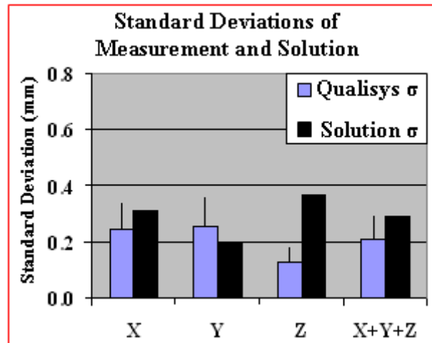
Figure 32. Graph of the measurement and solution error per-axis, as well as the average for all three axes. The dispersion bars on the Qualisys bars have a height equal to 0.41 times that of the bar height. Thus, a Qualisys bar and its respective dispersion bar have a combined height equal to the 1.41 error constraint.
