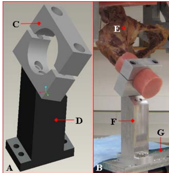
Figure 19. Schematic of the femur fixture assembly (A) and a photograph of it in use in the hip simulator (B). In the photograph, the femur fixture assembly (F) is attached to the x-y table (G) below, and to the femur of a cadaveric specimen (E).
