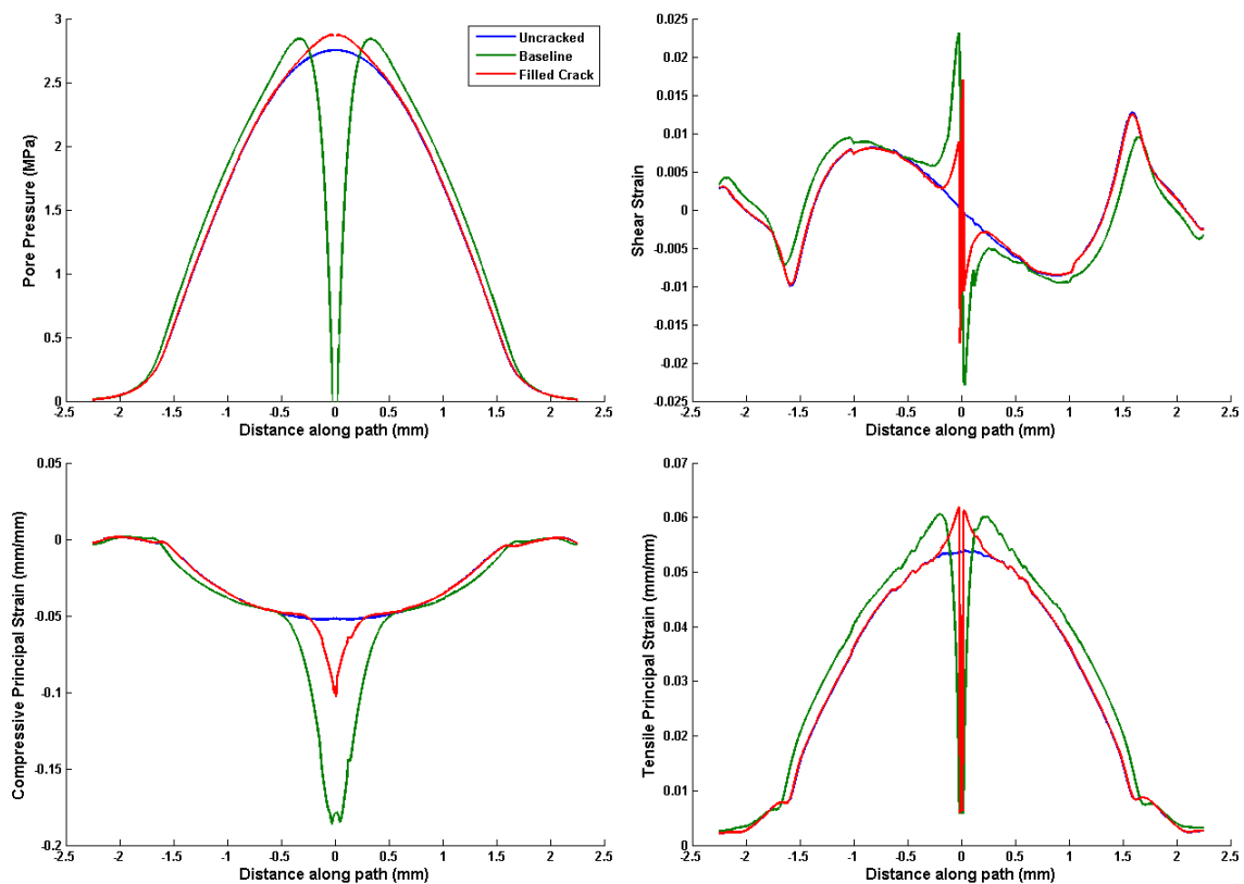
Figure 77. Fluid pressure and strains 100 \mu\text{m} below the articular surface in the filled crack model.
