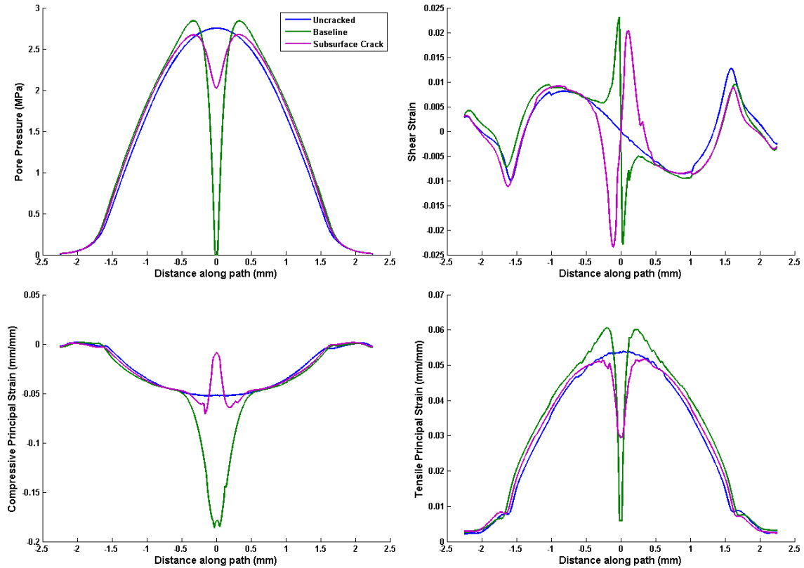
Figure 76. Fluid pressure and strains 300 \mu\text{m} below the articular surface in the subsurface model.
