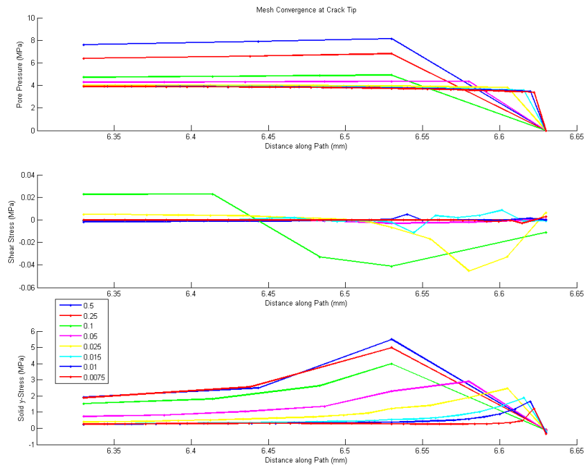
Figure 64. Mesh convergence approaching the tip. Element sizes 0.5 down to 0.015 represent global criteria, while 0.01 and 0.0075 are local refinements.
