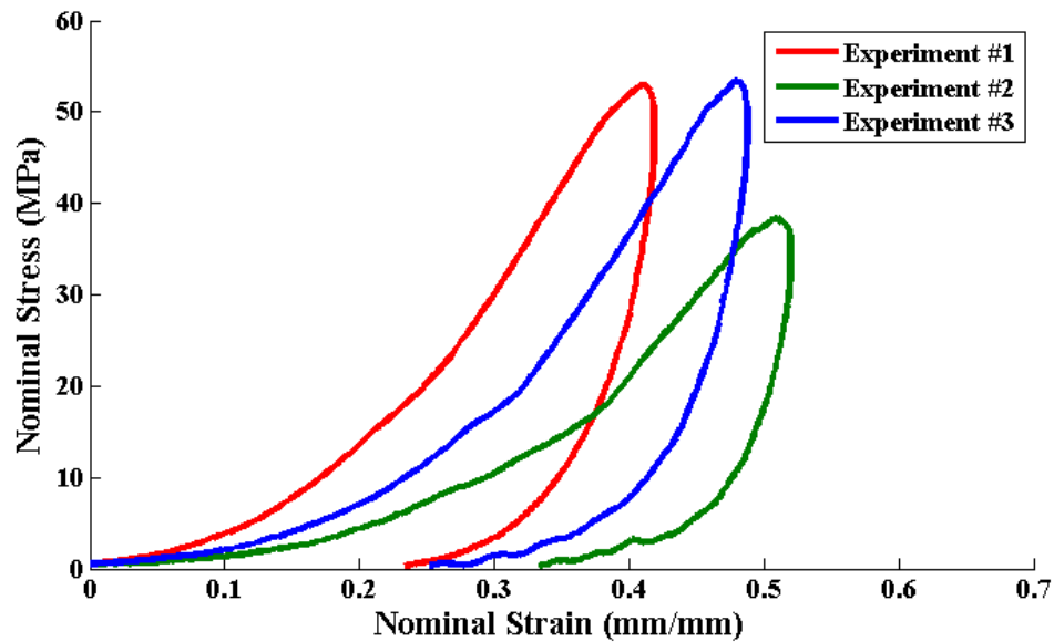
Figure 4. Representative stress-strain curves from impacts of bovine osteochondral explants.
