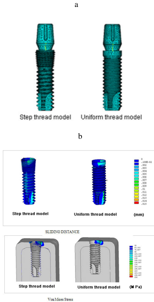
Figure 8. Result Of Finite Element Analysis
