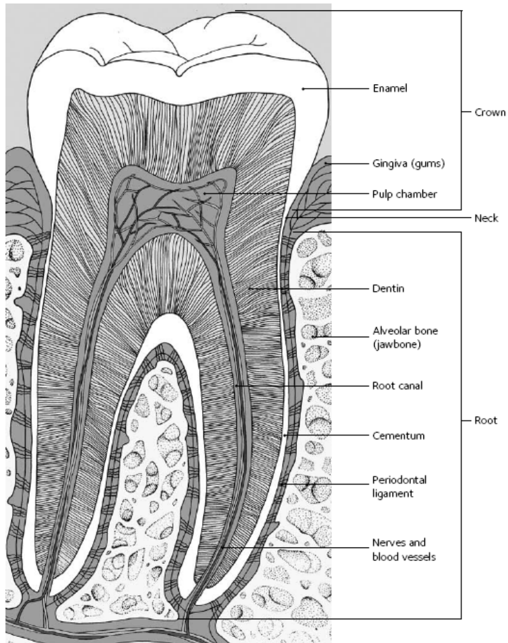
Figure 4. Tooth Anatomy
