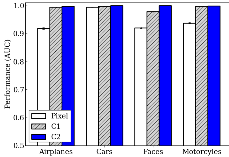
(a) Datasets from Fergus et al.
