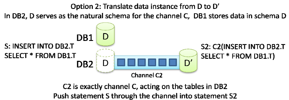
Figure 3.7: Using a channel and an insert statement to move entire instance of a table through a channel
