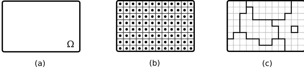
Figure 2.1. (a) Rectangular domain \Omega . (b) The domain is partitioned into cells \{\Omega_i\} with centers \{\mathbf{x}_i\} , i \in I . (c) Example partition of \Omega into six regions. Note that region boundaries always go along cell boundaries.
