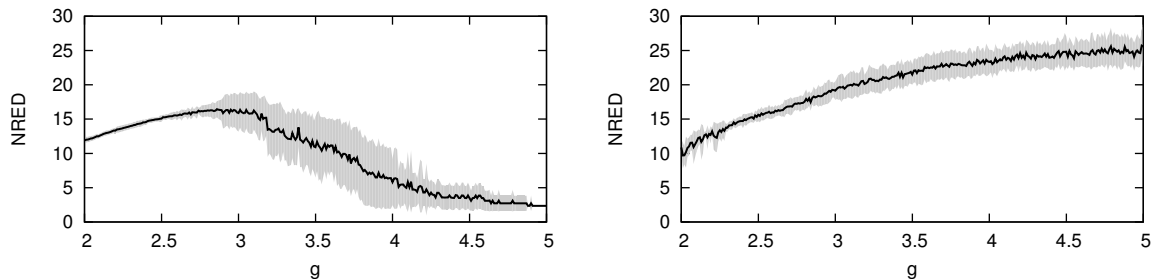
Figure 6.4. Noise reduction vs. parameter value with an algorithm using F_1 and the embedding depicted in Figure 6.5. The curve on the left corresponds to Figure 6.2 a), the curve on the right to Figure 6.2 c) (right column). The solutions for test case 3 are now excellent, while the solutions for test case 1 degrade and test case 4 (not shown) degrade slightly.
