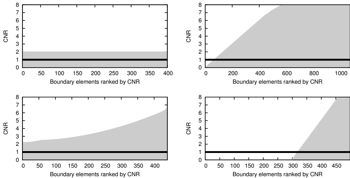
Figure 4.2. CNR over boundary elements for the test images 1 (upper left) to 4 (lower right) shown in Figure 4.1. CNR values above 8 are not shown.
