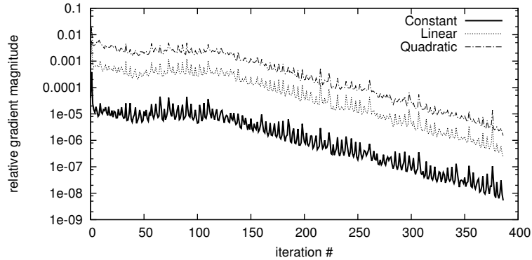
Figure 4.11. Development of the quantities \|(\nabla F_0(\mathbf{u}, s))_{-,k}\|_2 / \max(1, \|\mathbf{u}_{-,k}\|_2) for constant, linear, and quadratic coefficients, respectively, over iterations of the inner-loop in the minimization of objective function F_0 with test case 3. The notation \mathbf{u}_{-,k} denotes the vector consisting of the k -th coefficients in vector \mathbf{u} .
