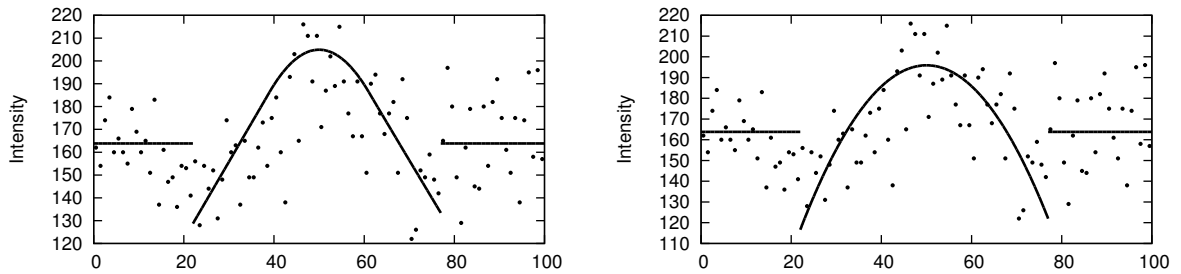
Figure 4.12. Example showing different results for test case 3 obtained with different accuracy of the intermediate solutions computed in the inner-loop. For the result on the left gtol = 10^{-4} was used, for the result on the right gtol = 10^{-6} was used in (7.4). The values for parameters b and d were chosen differently than in Figure 4.7 and Figure 4.8 to demonstrate this phenomenon.
