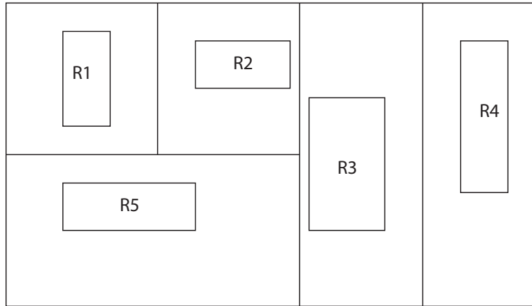
Figure 5.11: Maximal rectangles.
