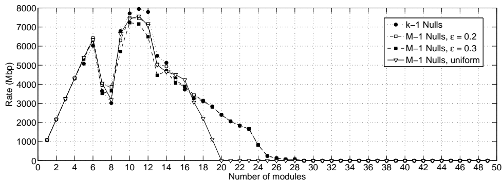
Figure 7.15: Maximum throughput with a circular array.
