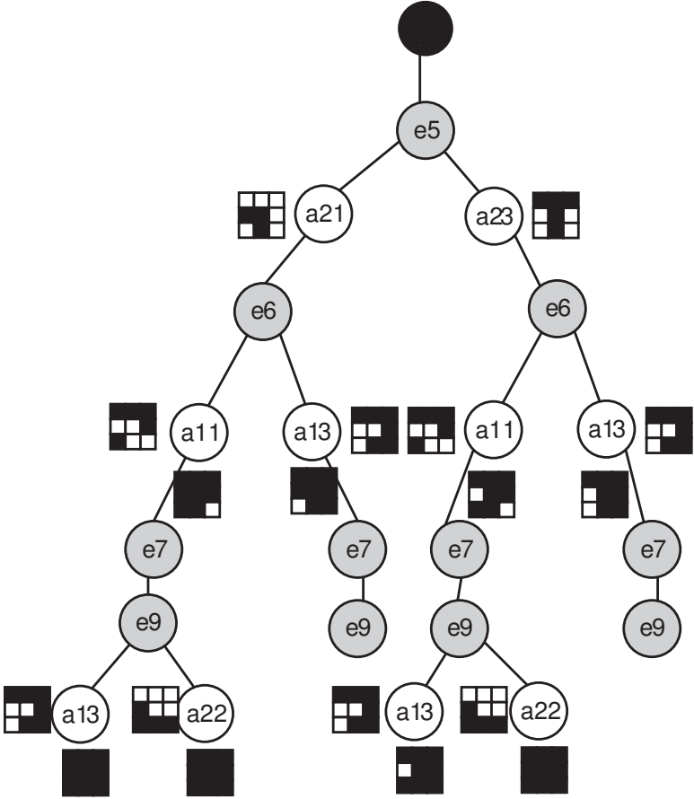
Figure 5.8: e5,e6,e7,e9 tree
