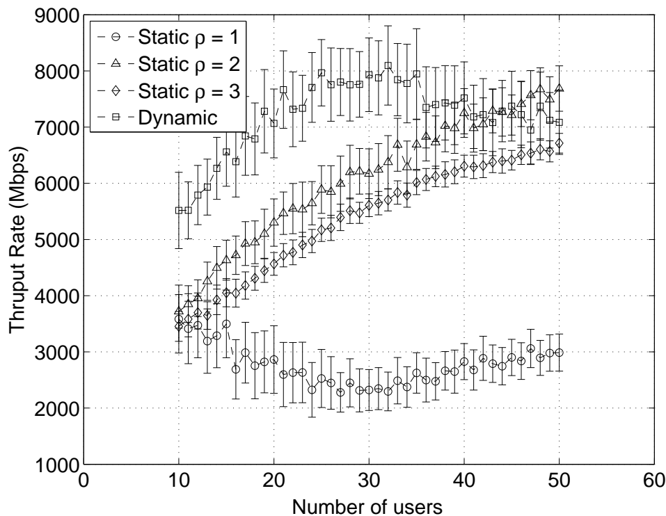
Figure 7.17: Average throughput.
