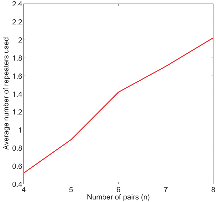
Figure 8.13: Average number of repeaters used.
