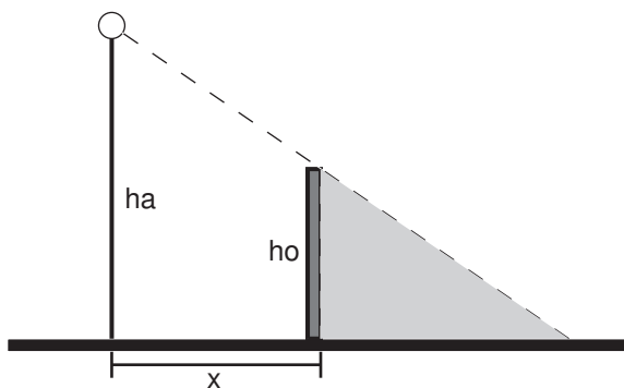
Figure 5.1: Relation between distance from antenna to obstruction and coverage
