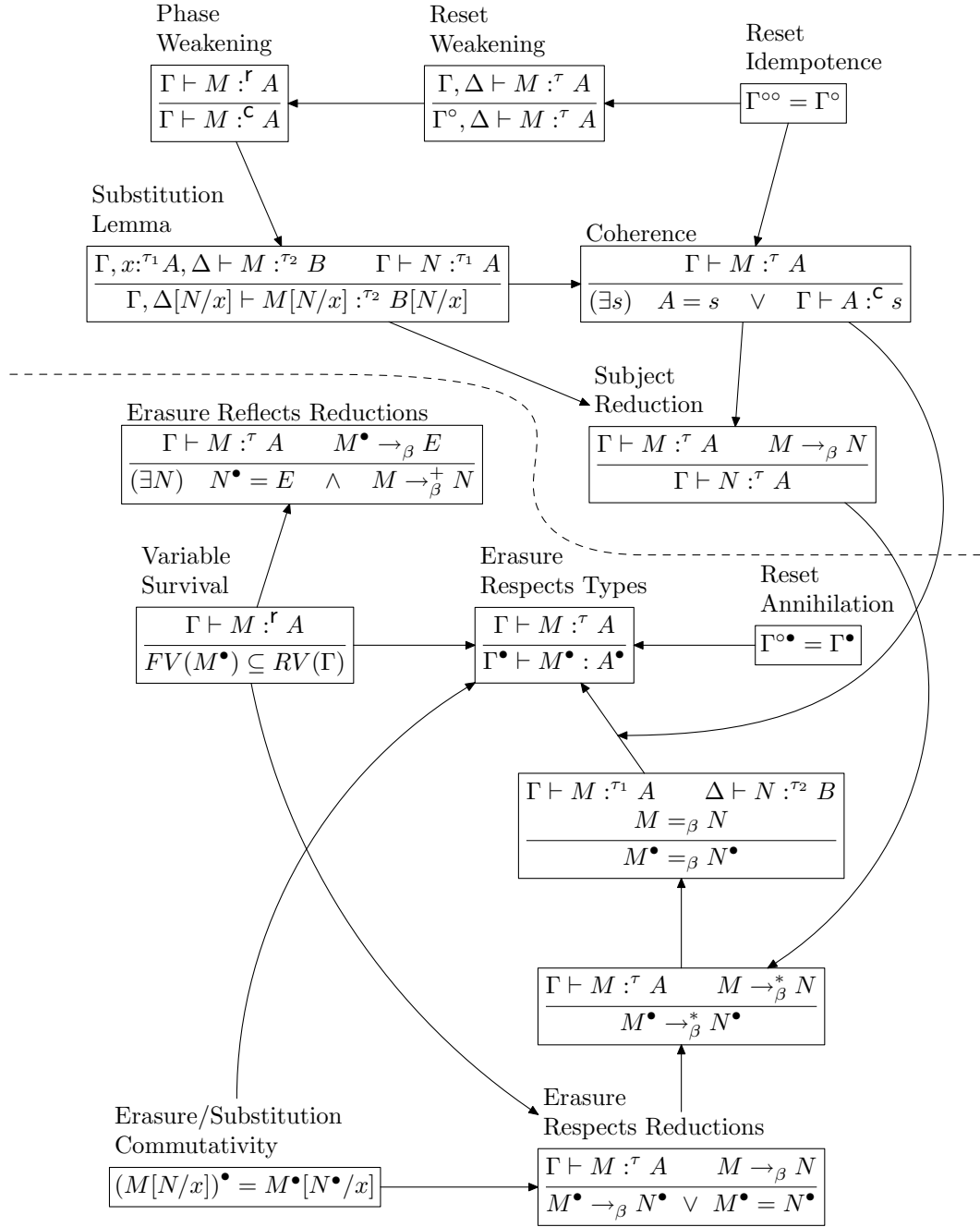
Figure 3.4: Identities and admissible rules in the meta-theory of EPTS (above the dotted line) and erasure (below it). Arrows indicate proof dependencies.
