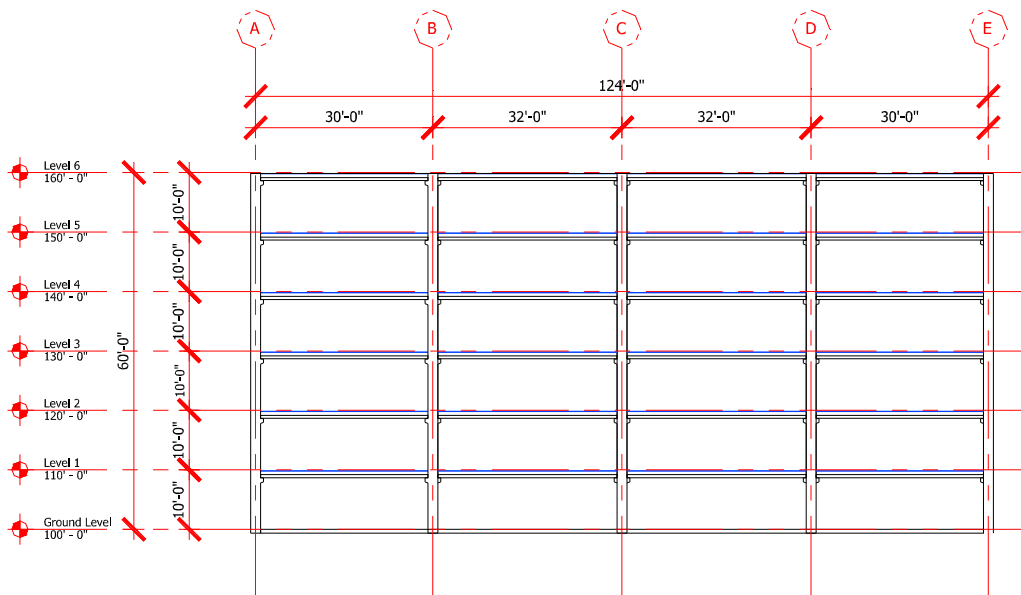
Figure 4.2 – Typical Building Section
