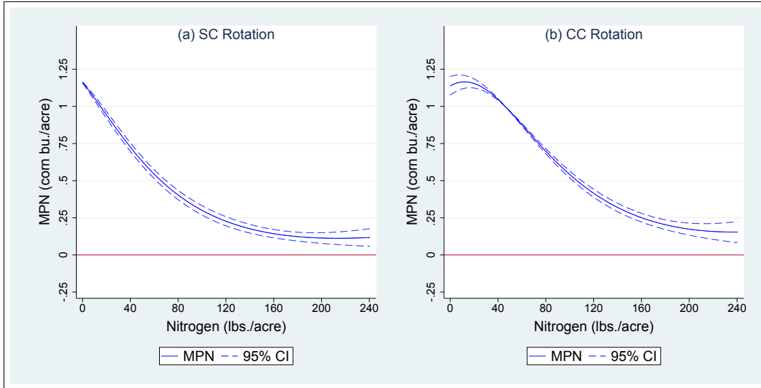
Figure 3.4 MPN conditional on nitrogen and weather for the Ames farm: (50%-50%-50%) denotes a weather scenario with 50 th percentile of growing season rainfall, growing season degree days and pre-season precipitation respectively.
