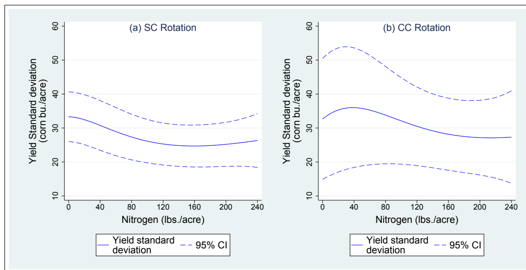
Figure 3.13 Yield standard deviation conditional on nitrogen for the Ames farm under weather uncertainty.
