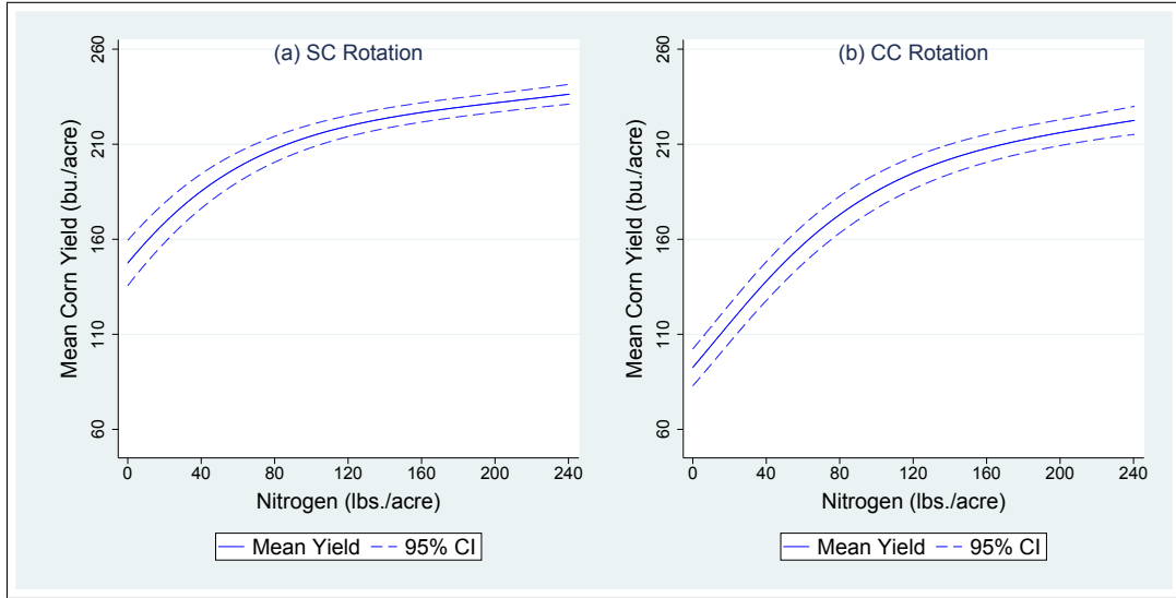
Figure 3.3 Mean Yield conditional on nitrogen and weather for the Ames farm: (50\%-50\%-50\%) denotes a weather scenario with the 50 th percentile of the growing season rainfall, the TDD and the pre-season precipitation respectively.
