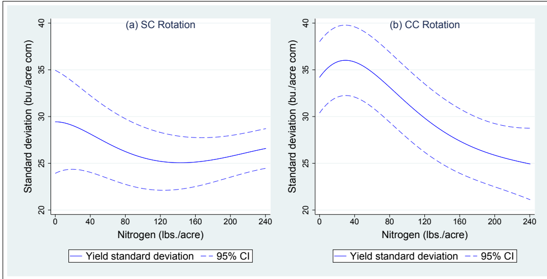
Figure 3.12 Standard deviation of yield conditional on nitrogen and weather for the Ames farm: (50\%-50\%-50\%) denotes a weather scenario with the 50 th percentile of growing season rainfall, the TDD and the pre-season precipitation respectively.
