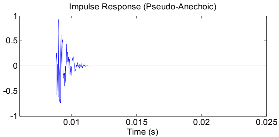
Figure 2.2: Pseudo-anechoic impulse response.
