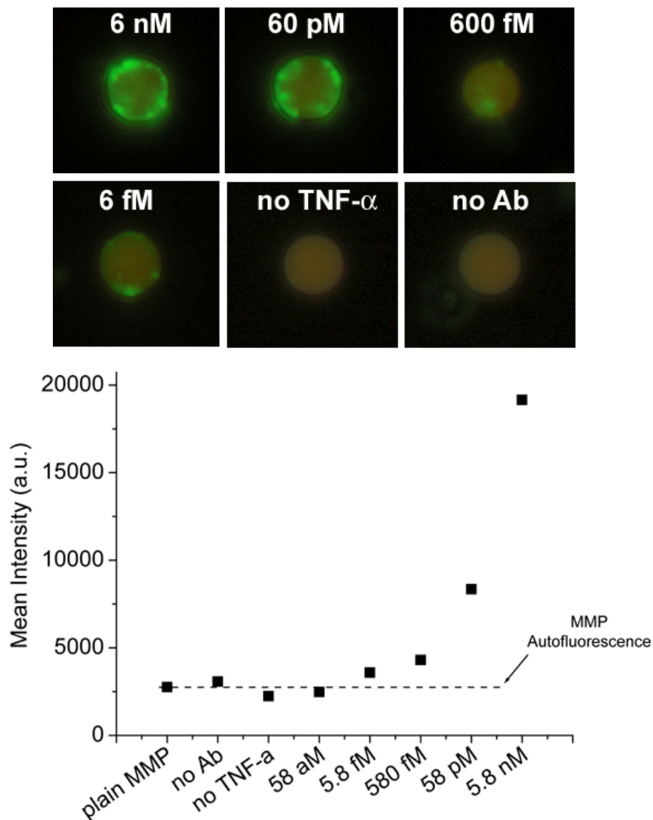
Figure 4.4: Single-bead immunoassay for TNF-alpha detection using luminescent nanoparticles (dye-doped particles). Fluorescence microscope images (top figure) obtained at varying concentrations of target. Plot of the integrated fluorescence intensity as a function of target concentration (bottom figure). Spectral shift of nanoparticles from bead autofluorescence is evident.
