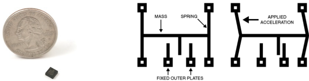
Figure 17: MEMS accelerometer case Figure 18: MEMS accelerometer mechanism
