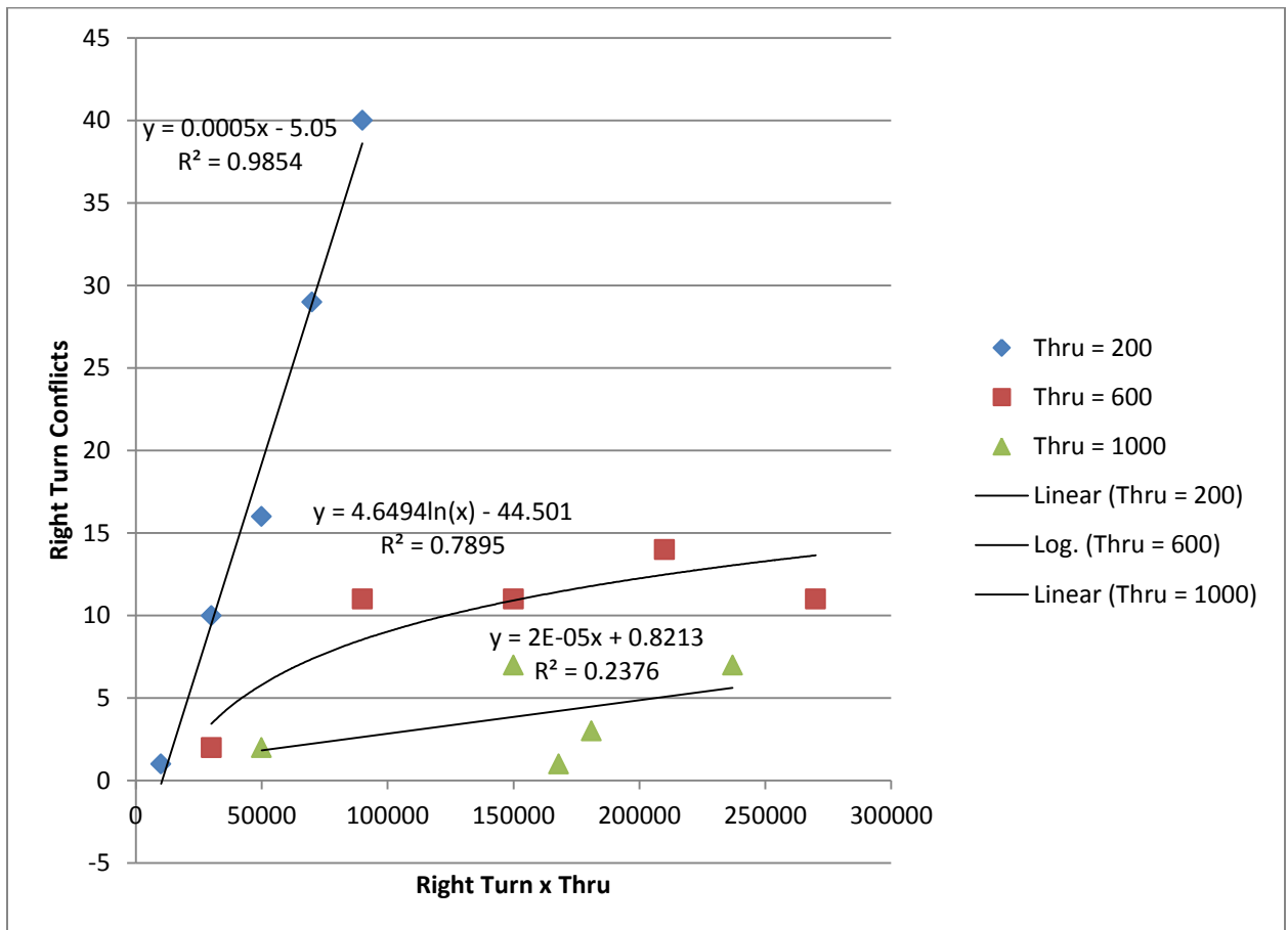
Figure 8: Right-turn Conflicts by Right Turn Volume x Through Volume (1 Lane)
