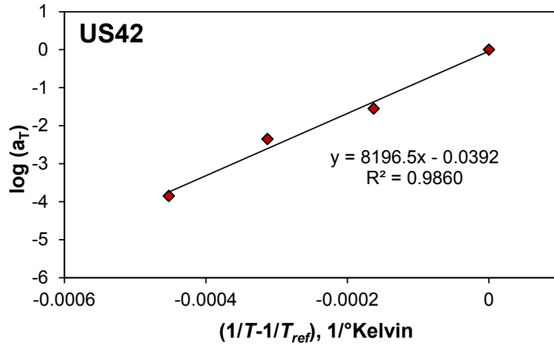
Figure A.9. Shift Factors and Arrhenius Function for US42 Mix
