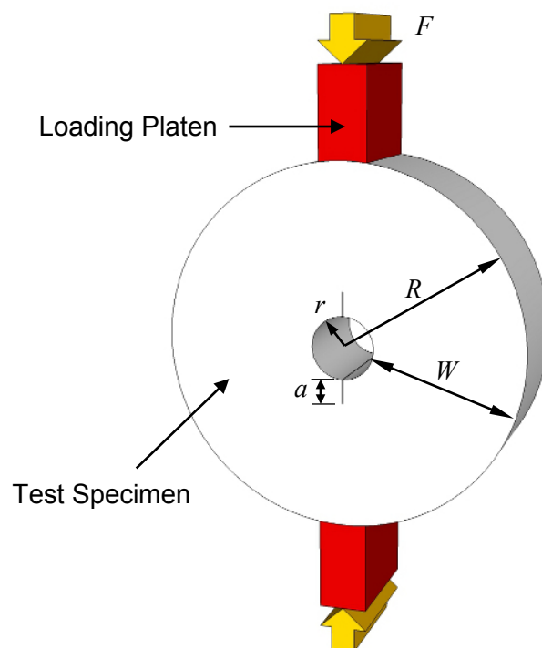
Figure 1.8. Indirect Ring Tension Fracture Test Geometry
