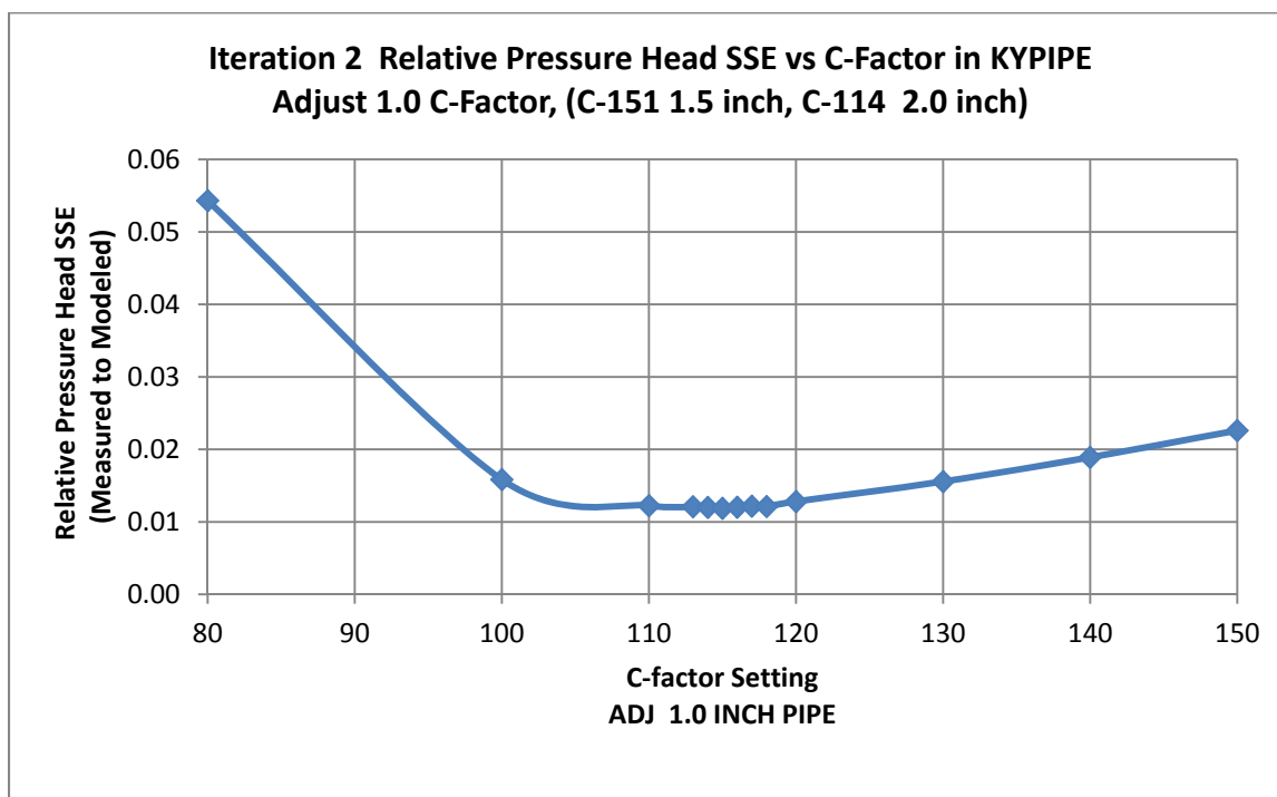
Figure B.7: Case B pressure head calibration, Iteration two, 1.0 pipe adjustment
