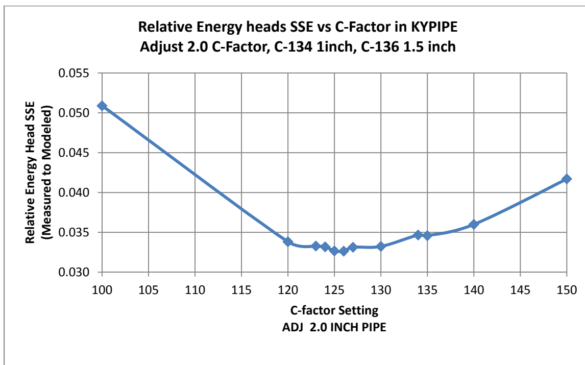
Figure A.16: Case A energy head calibration, 2.0 pipe adjustment
