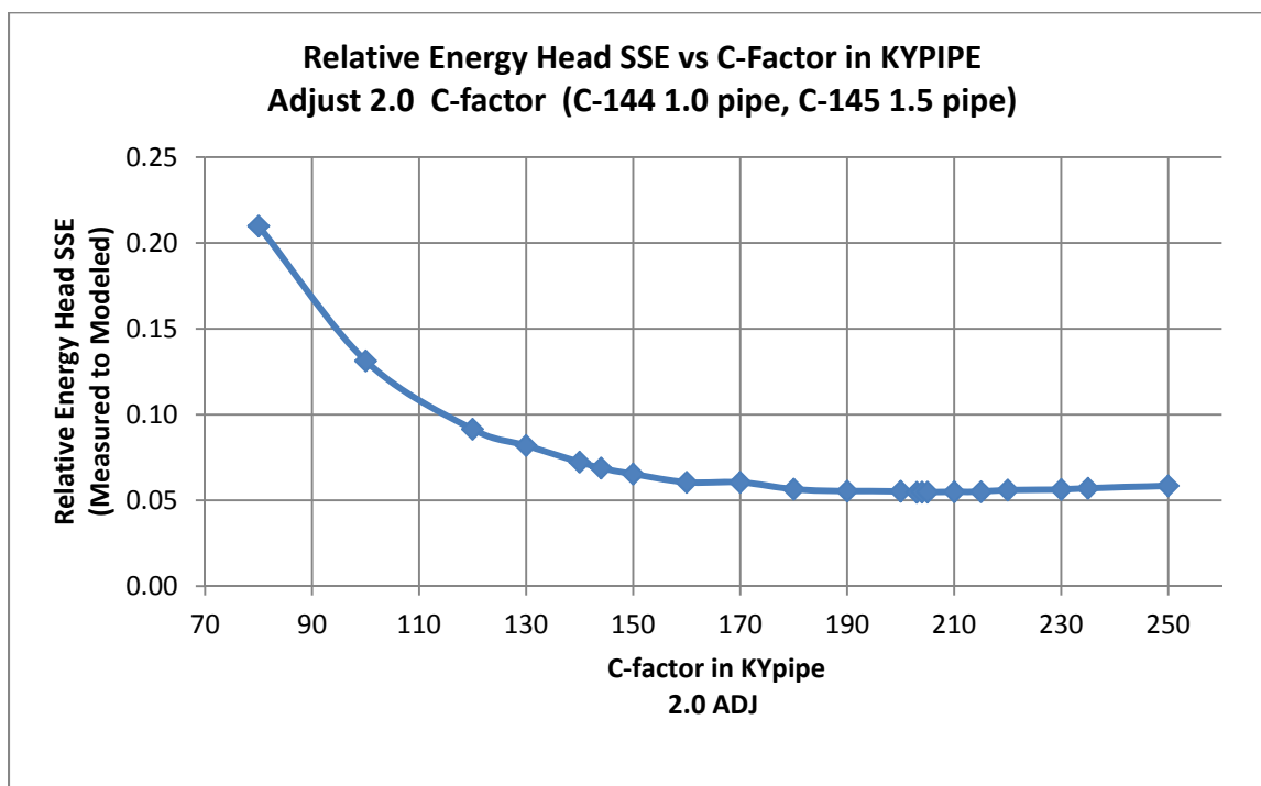
Figure B.21: Case B energy head calibration, 2.0 pipe adjustment
